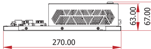
Rear View
