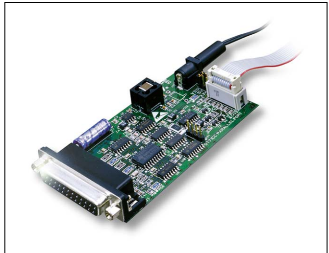
Figure 1: ST7-STICK Programmer
