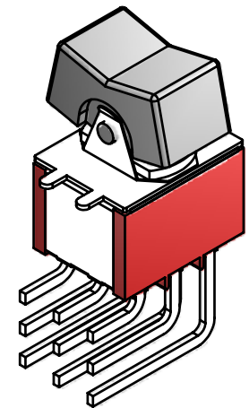
ISOMETRIC
