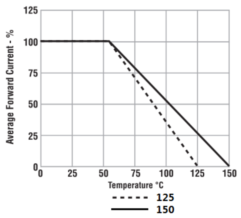
Forward Current Derating Curve
