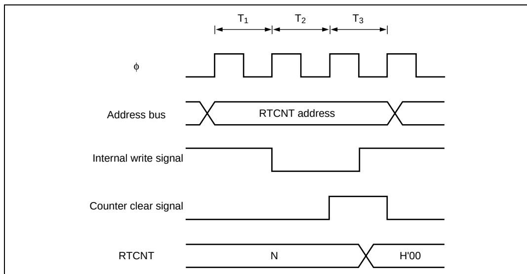
Figure 6.39 Contention between RTCNT Write and Clear
