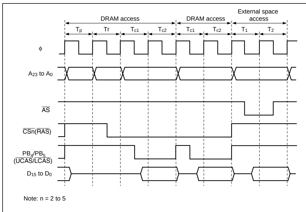
Figure 6.25 Example of Operation Timing in RAS Up Mode
