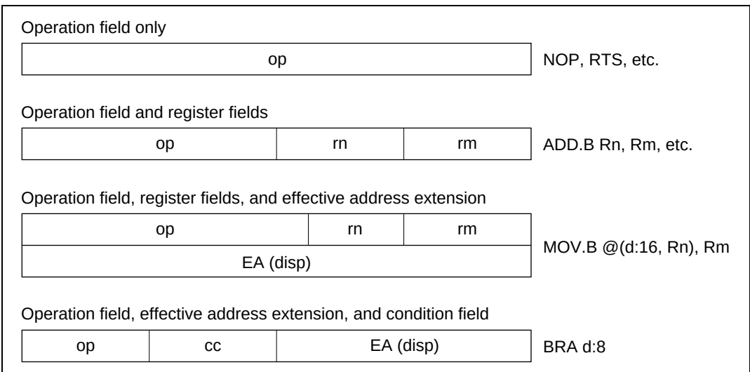
Figure 2.9 Instruction Formats
