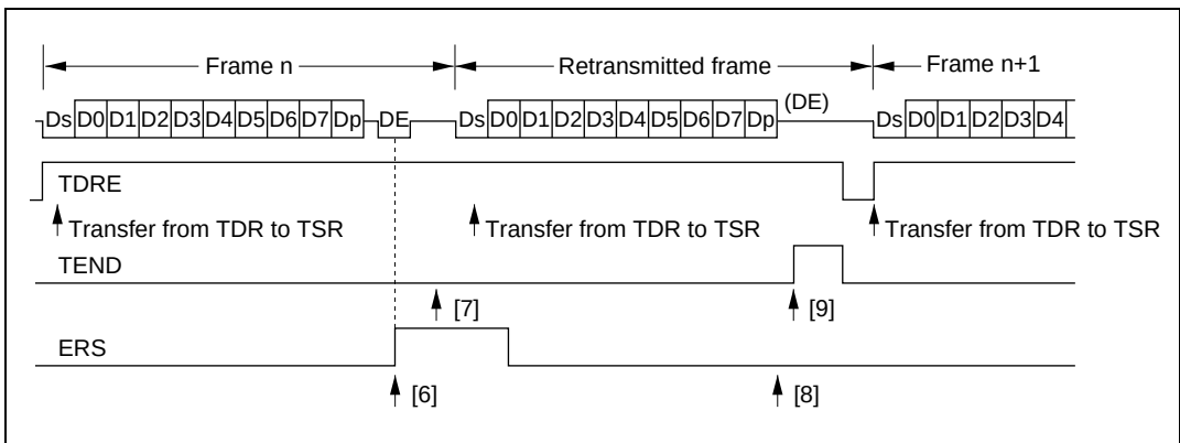
Figure 14.13 Retransmission in SCI Transmit Mode
