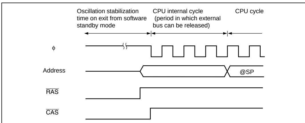
Figure 6.37 Self-Refresh Clearing
