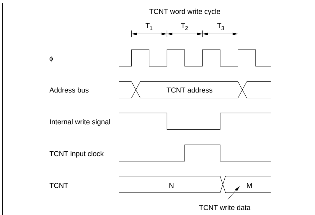
Figure 9.38 Contention between TCNT Word Write and Increment
