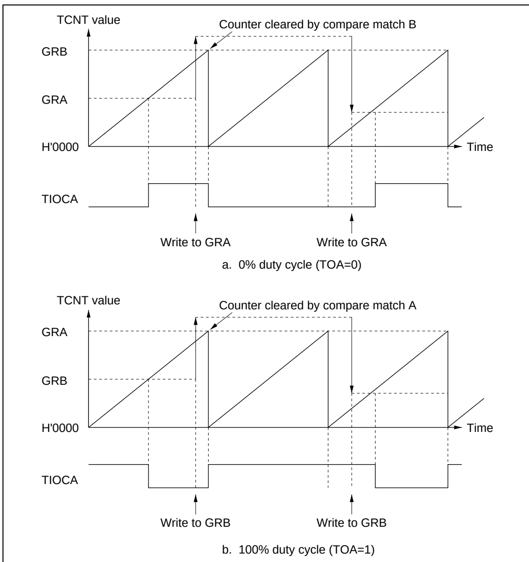
Figure 9.28 PWM Mode (Example 2)
