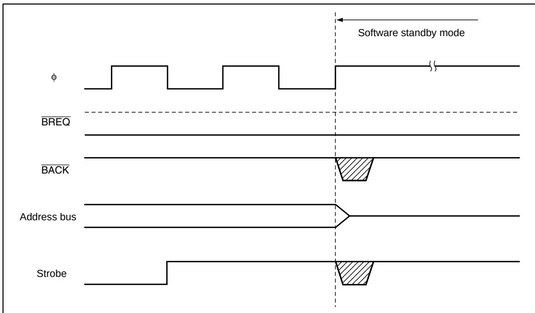
Figure 6.36 Bus-Released State and Software Standby Mode
