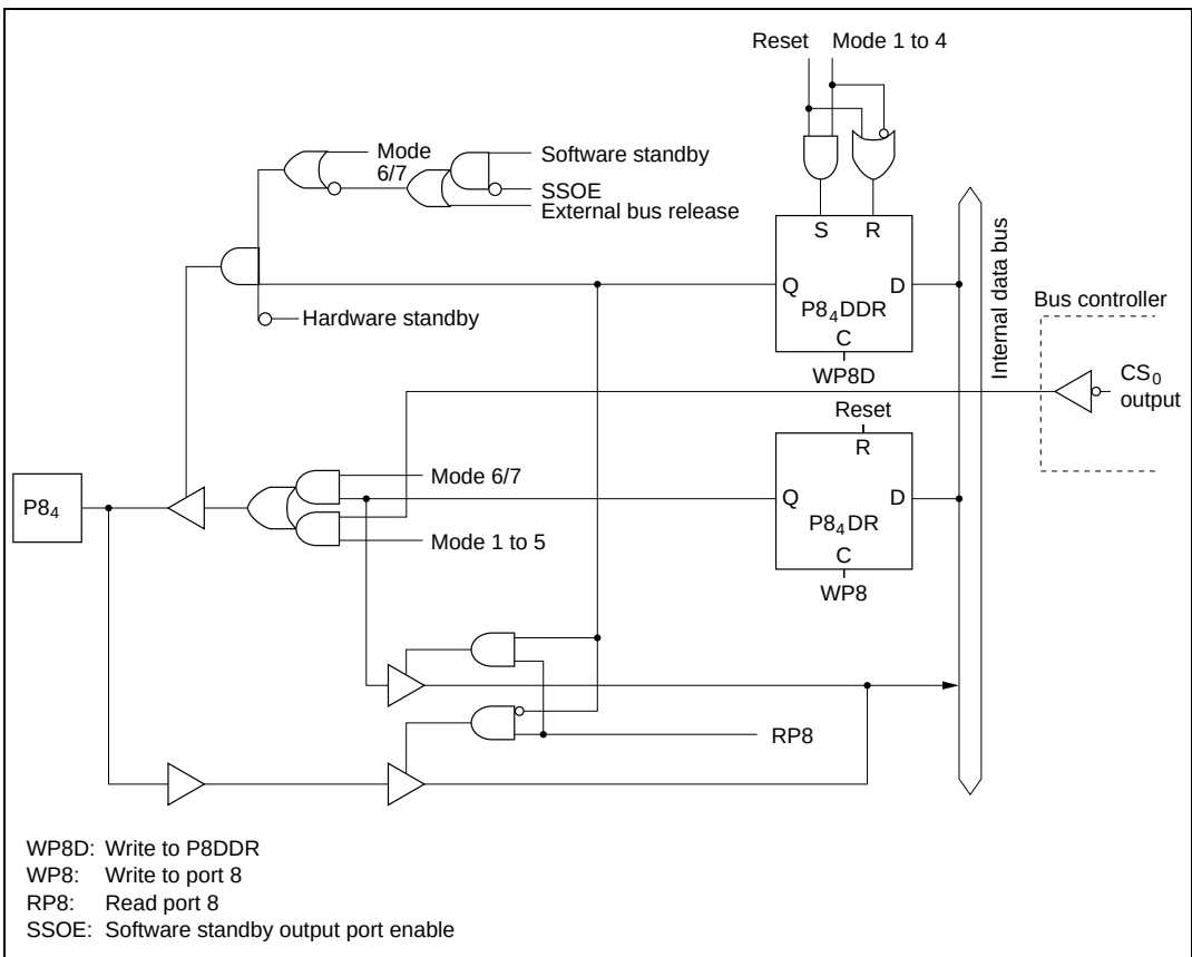
Figure C.8 (e) Port 8 Block Diagram (Pin P84)
