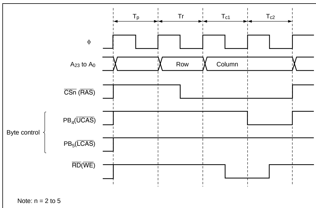
Figure 6.21 Control Timing (Upper-Byte Write Access When CSEL = 0)
