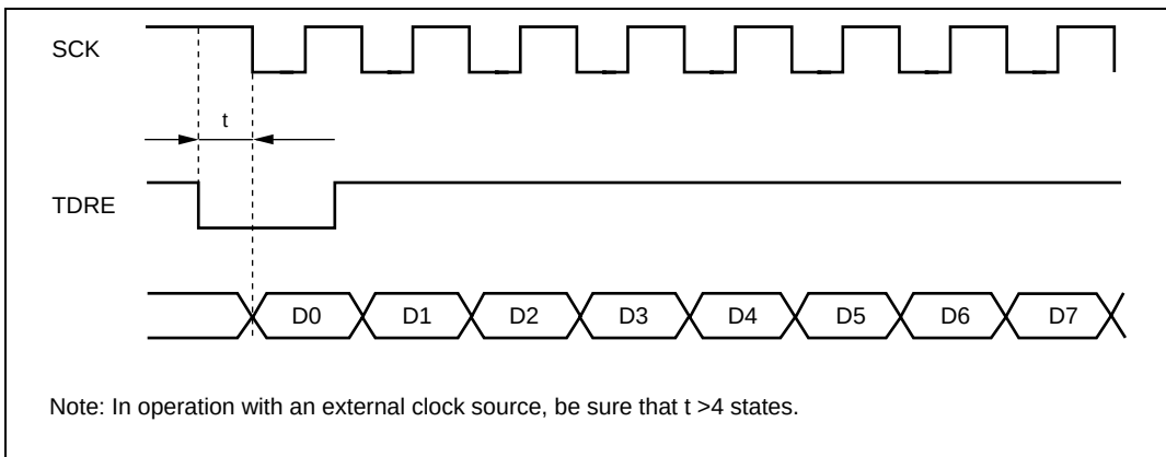
Figure 13.22 Example of Synchronous Transmission Using DMAC
