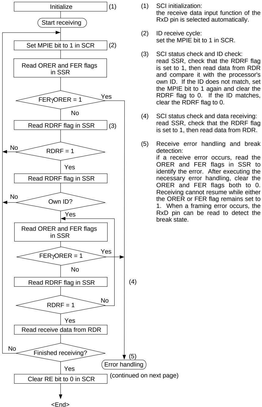
Figure 13.12 Sample Flowchart for Receiving Multiprocessor Serial Data (1)
