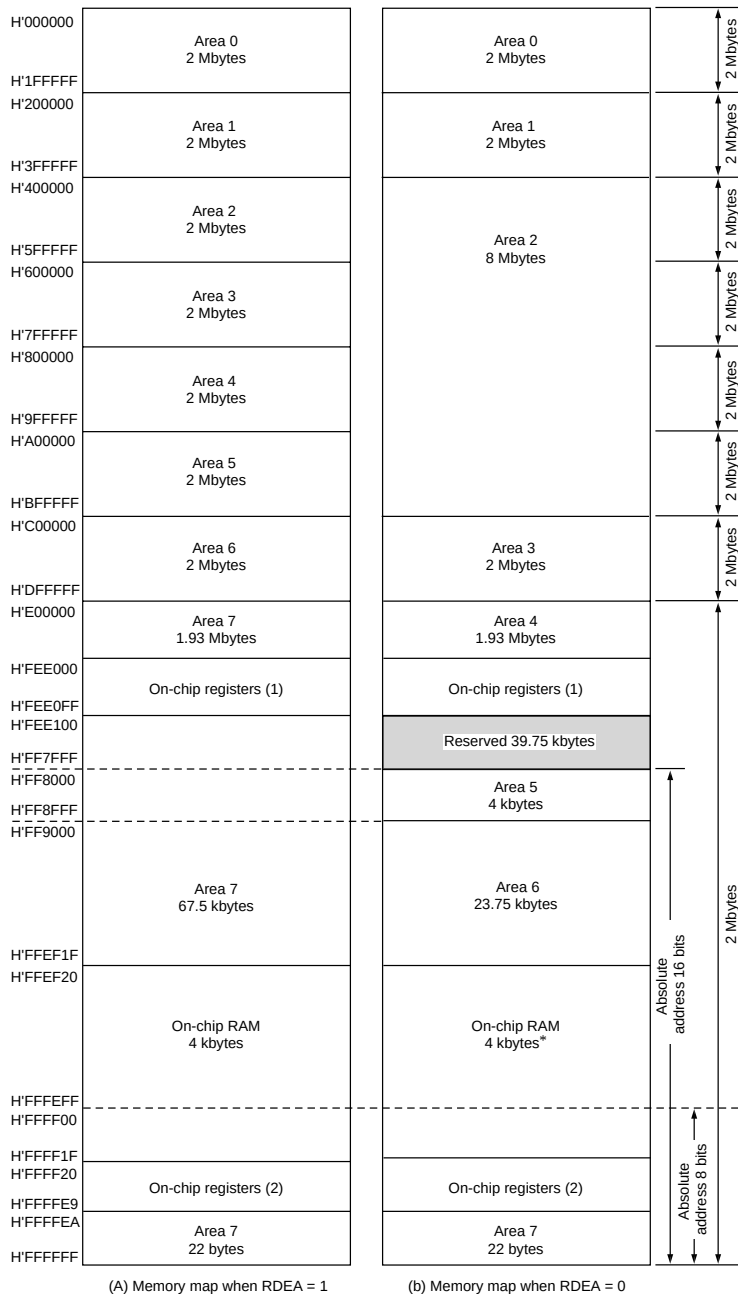
Figure 6.3 Memory Map in 16-Mbyte Mode (H8/3067, H8/3066)
