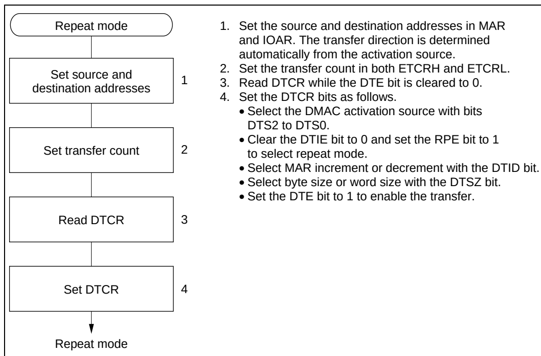
Figure 7.7 Repeat Mode Setup Procedure (Example)
