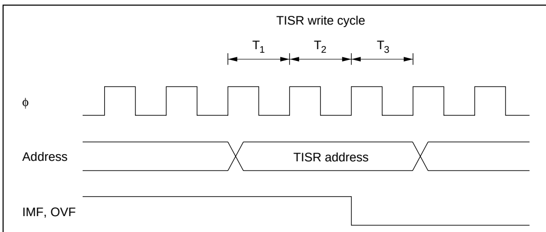
Figure 9.36 Timing of Clearing of Status Flags
