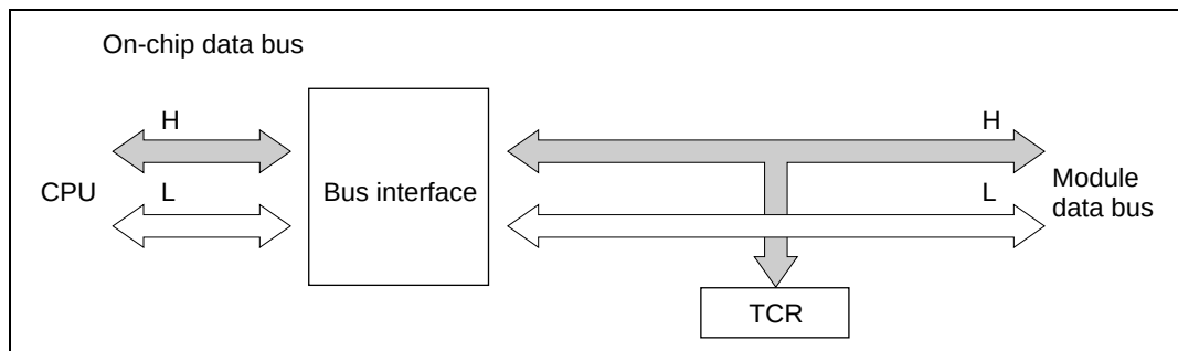
Figure 9.10 TCR Access (CPU Writes to TCR)
