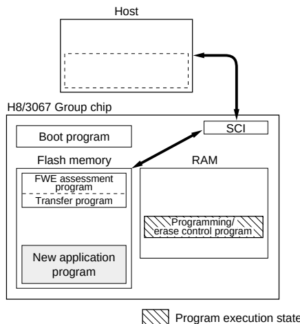
Figure 18.4 User Program Mode (Example)
