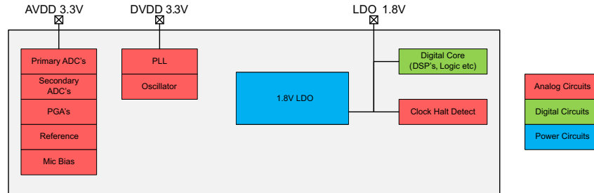
Figure 77. Power Distribution Tree within PCM5252
