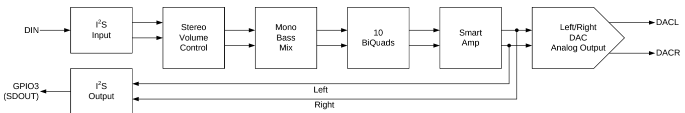
Figure 60. Example Processflow
