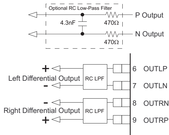
Figure 61. Optional Low Pass Filters
