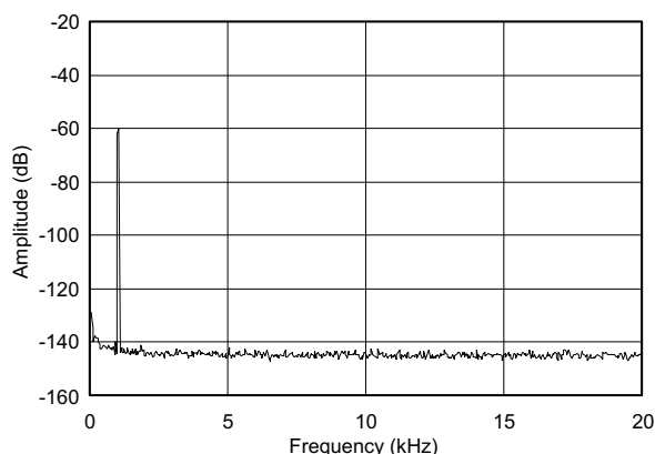
Figure 76. 2 FFT Plot At -60db Input
