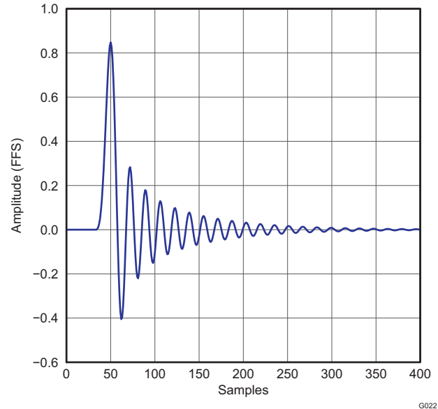
Figure 34. Low latency x8 Interpolation Filter Impulse Response
