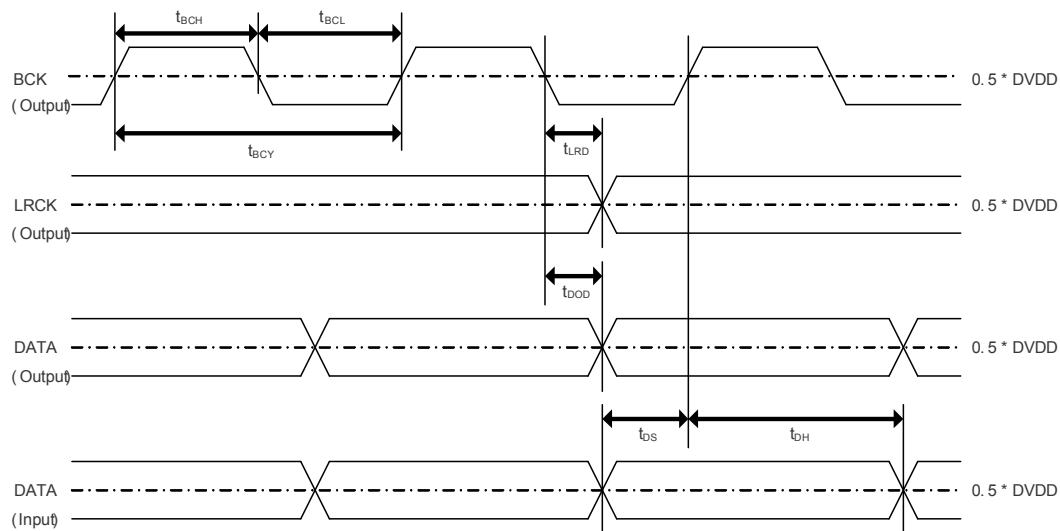
Figure 6. PCM5252 Serial Audio Timing - Master
