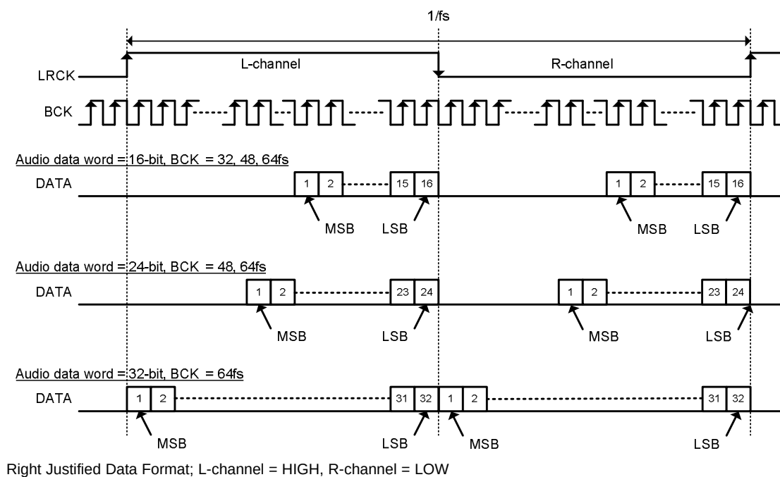
Figure 20. Right Justified Audio Data Format
