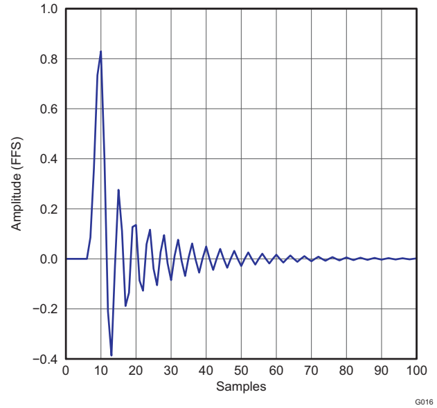
Figure 40. Low latency \times 2 Interpolation Filter Impulse Response
