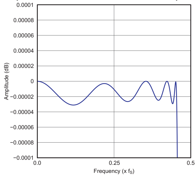
Figure 41. Low latency \times 2 Interpolation Filter Passband Ripple
