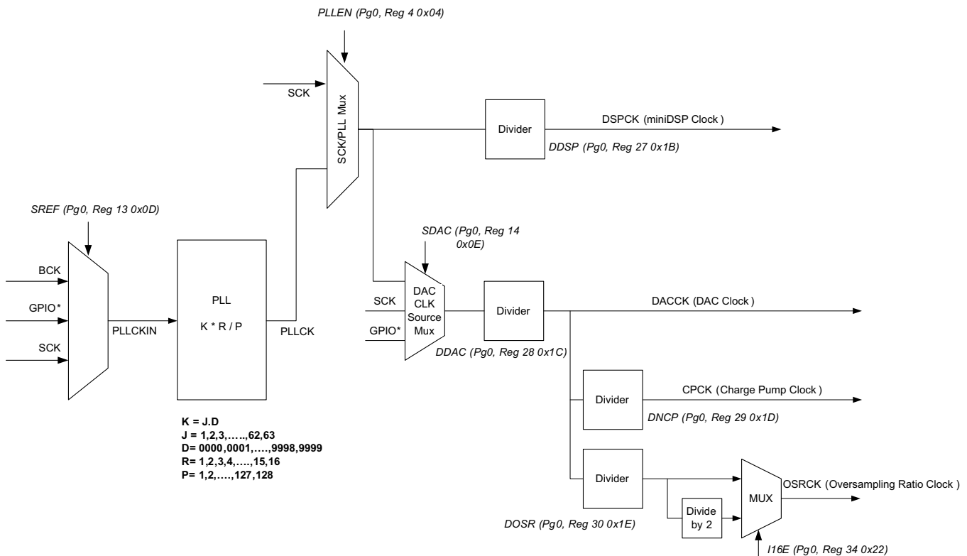
Figure 63. PCM5252 Clock Distribution Tree
