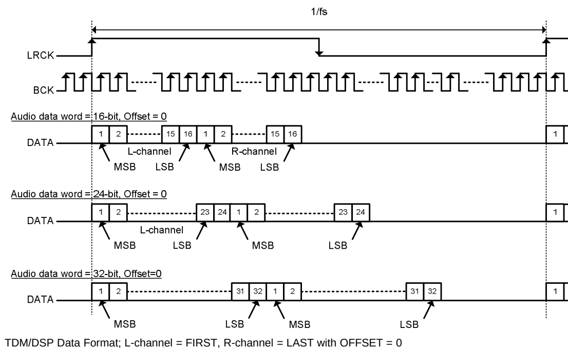
Figure 21. TDM/DSP 1 Audio Data Format
