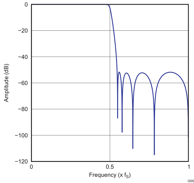
Figure 39. Low latency \times 2 Interpolation Filter Frequency Response
