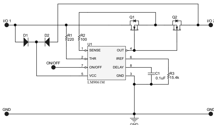
Figure 22. Bidirectional Switch
