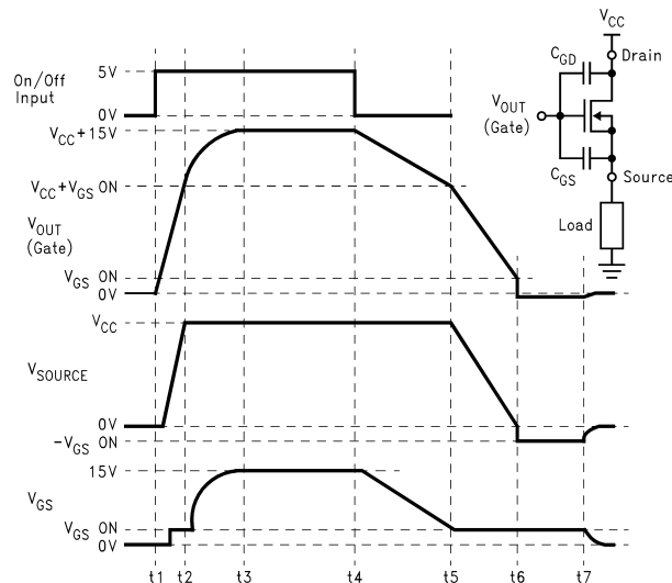
Figure 13. Turnon and Turnoff Waveforms
