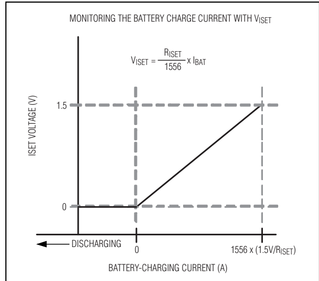
Figure 5. Monitoring the Battery Charge Current with ISET Output Voltage
