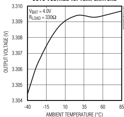
OUT5 VOLTAGE vs. TEMPERATURE
