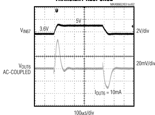
OUT6 REGULATOR LINE-TRANSIENT RESPONSE
