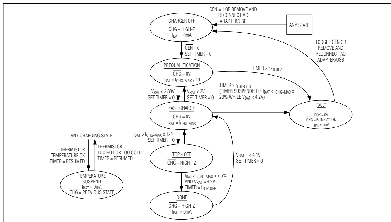
Figure 4. Charger State Diagram
