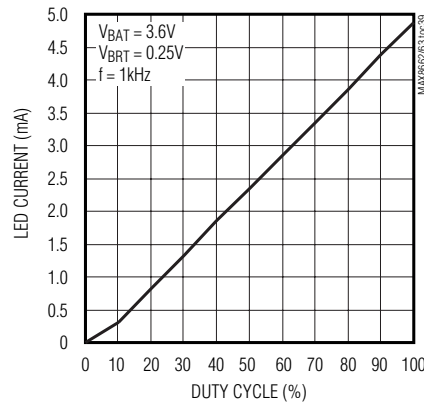
LED CURRENT vs. PWM DIMMING DUTY CYCLE
