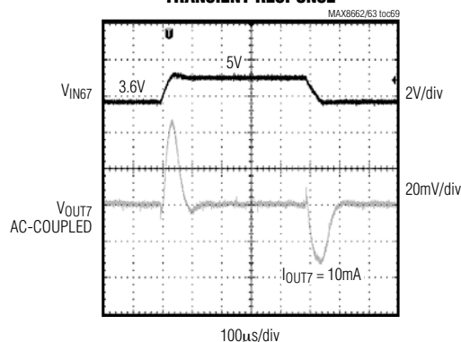
OUT7 REGULATOR LINE-TRANSIENT RESPONSE
