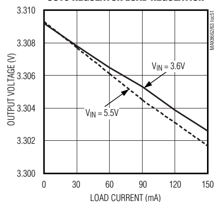
OUT5 REGULATOR LOAD REGULATION
