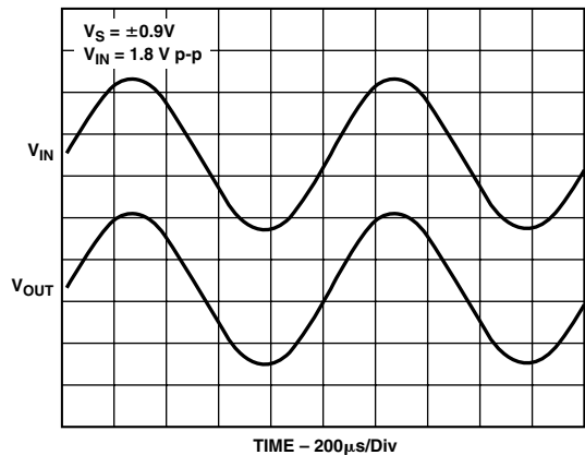
Figure 20. Rail-to-Rail Input Output
