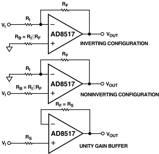
Figure 21. Input Bias Cancellation Circuits
