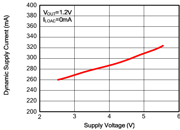
Dynamic Supply Current vs Supply Voltage
