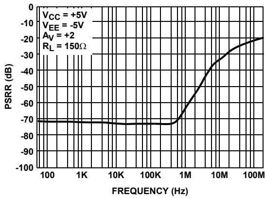
FIGURE 13. PSRR ( V_{EE} )
