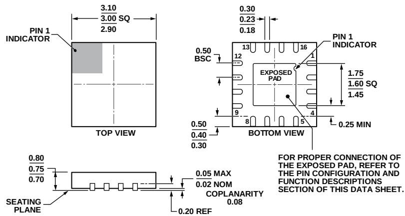
Figure 60. 16-Lead Lead Frame Chip Scale Package [LFCSP_WQ] 3 mm × 3 mm Body, Very Very Thin Quad (CP-16-22)
