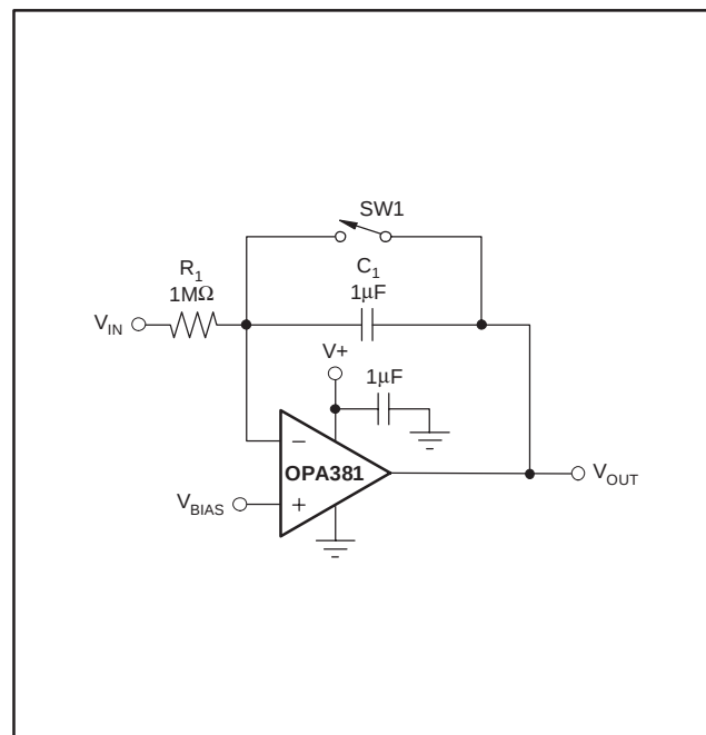
Figure 15. Precision Integrator
