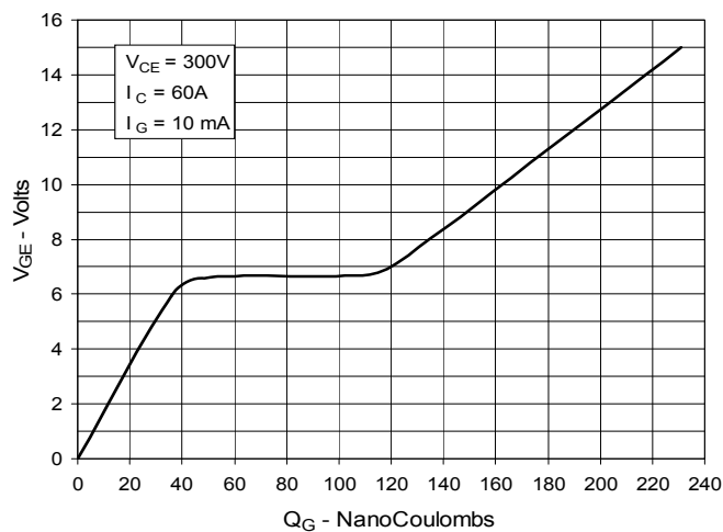
Fig. 8. Gate Charge
