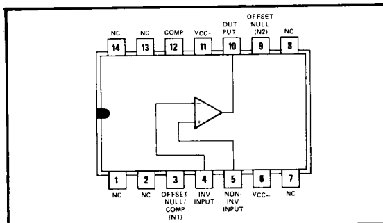
JG OR P DUAL-IN-LINE PACKAGE (TOP VIEW)
