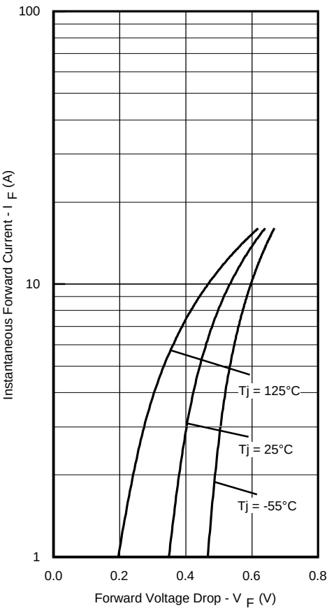
Fig. 1 - Max. Forward Voltage Drop Characteristics (Per Leg)
