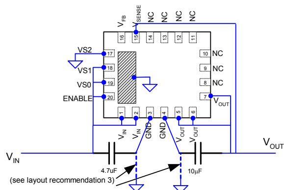
Figure 6. Example application, Vout=1.5V.
