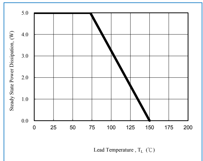
Figure 4 - Steady State Power Derating Curve
