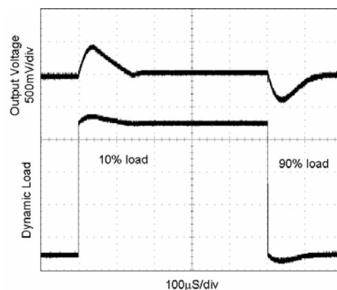
Figure 9. Typical V_{iso} Transient Load Response 5V Output 10%-90% Load Step
