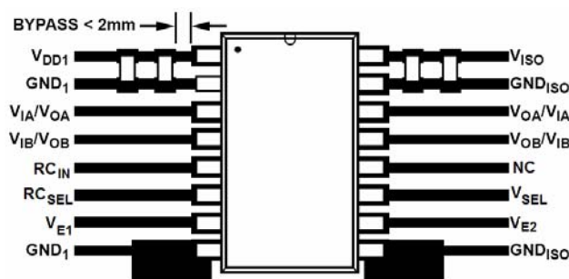
Figure 17. Recommended Printed Circuit Board Layout
