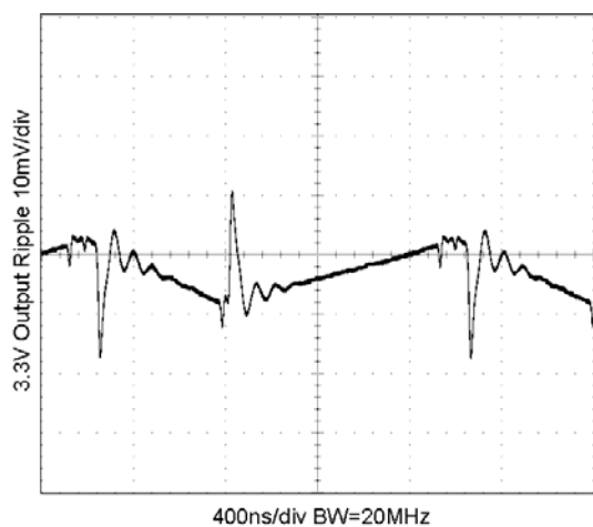
Figure 12. Typical V_{iso}=3.3V Output Voltage Ripple at 90% Load
