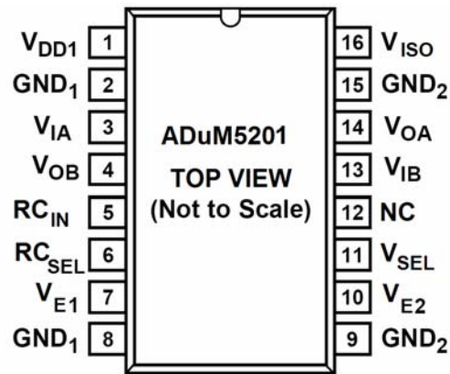
Figure 4. ADuM5201 Pin Configuration
