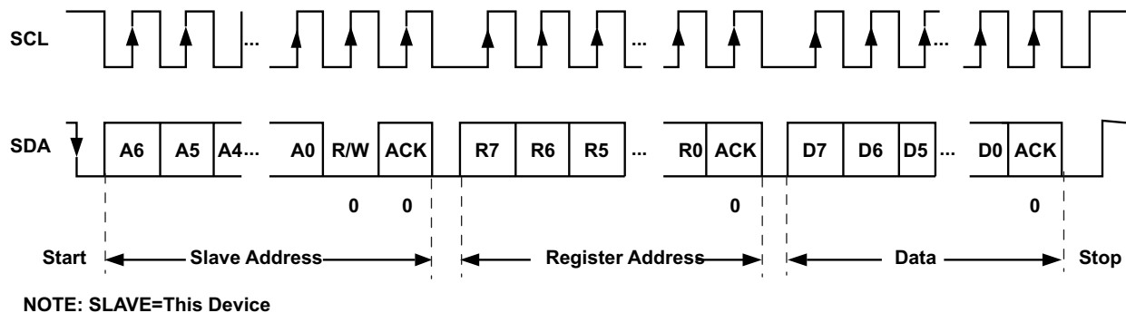
Figure 6-21. I²C Interface WRITE to Device in F/S Mode
