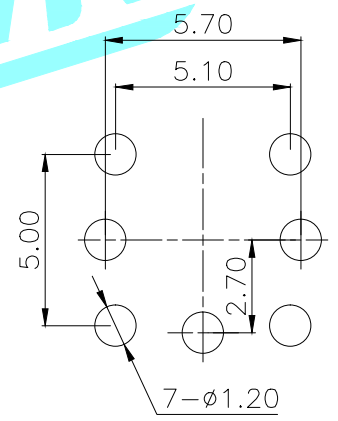
PCBLayout(Pattern Side)
