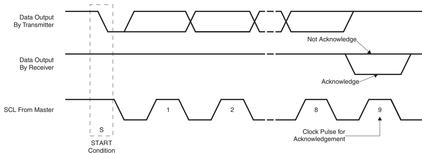
Figure 13. Acknowledge on the I²C Bus
