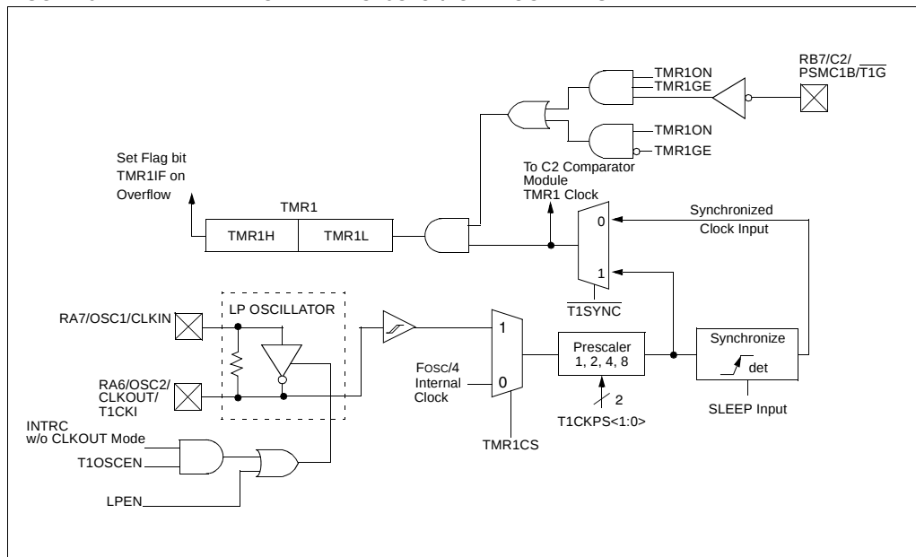
FIGURE 6-2: TIMER1 ON THE PIC16C781/782 BLOCK DIAGRAM
