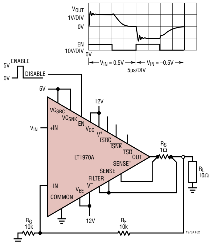
Figure 2. Using the ENABLE pin
