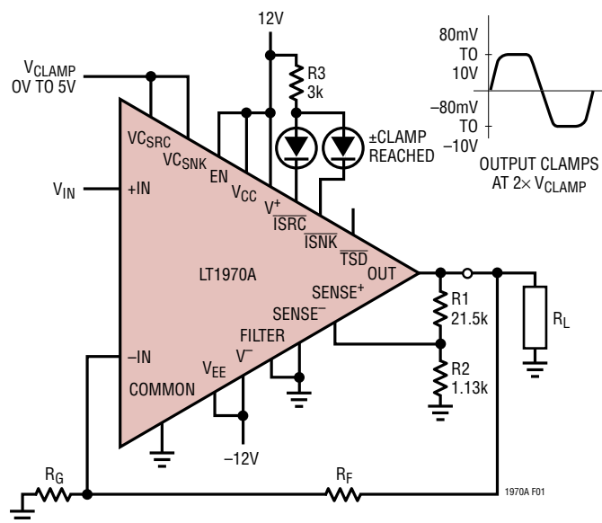
Figure 1. Symmetrical Output Voltage Limiting
