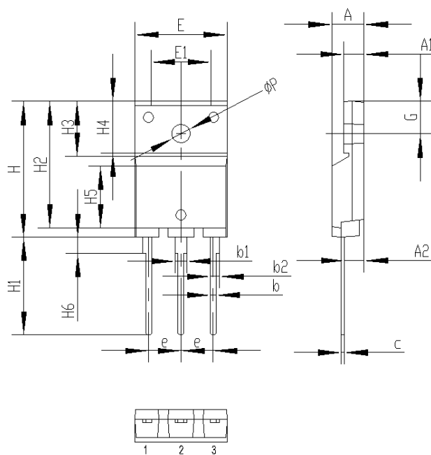
TO-3PF(TO-3PML) Outline
