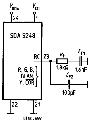
Test Circuit 3
