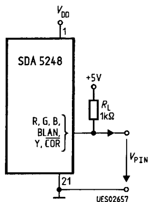
Test Circuit 1
