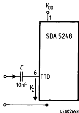
Test Circuit 2
