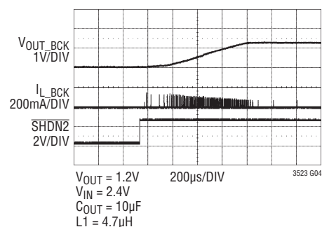
Inrush Current Control for the Step-Down Converter
