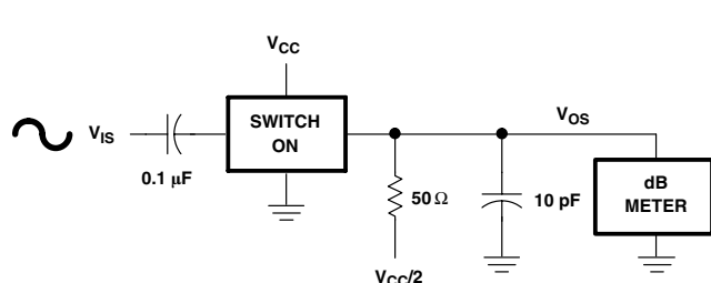
Figure 2. Frequency-Response Test Circuit
