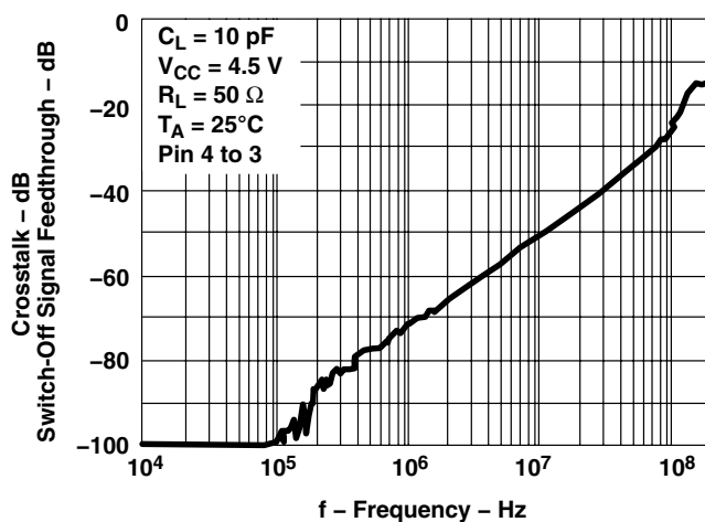
Figure 9. Switch-OFF Signal Feedthrough and Crosstalk vs Frequency, V_{CC} = 4.5 V
