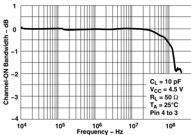
Figure 8. Switch Frequency Response, V_{CC} = 4.5 V
