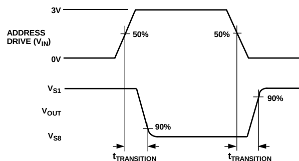
Figure 24. Switching Time of Multiplexer, t_{TRANSITION}
