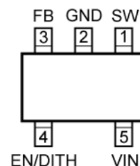
5-Pin Thin SOT-23 (D5) (Top View)
