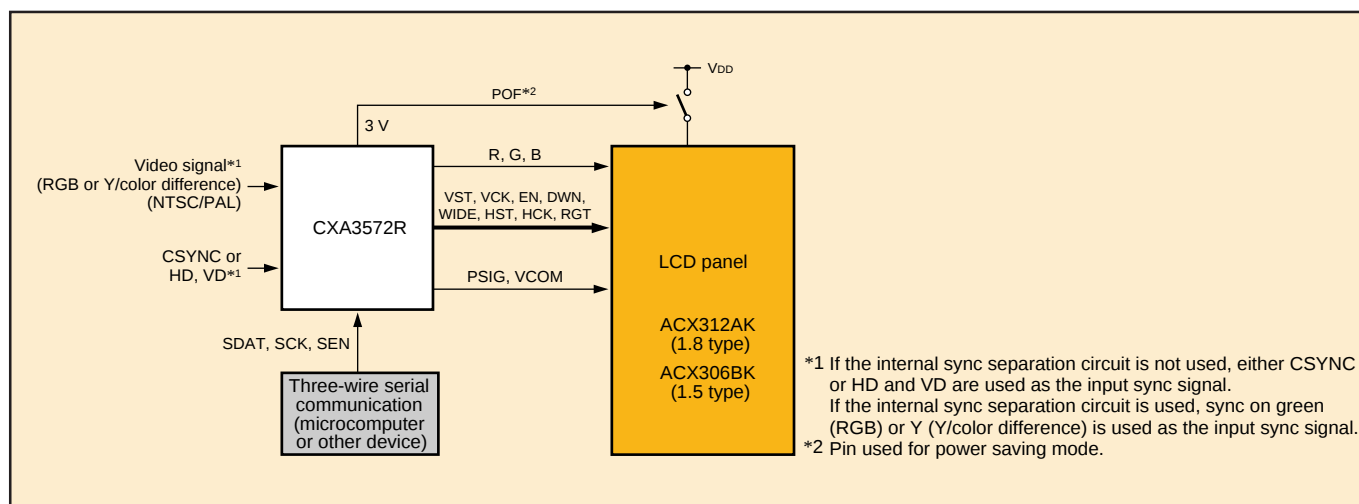
■ Figure 2 ACX312AK/306BK Drive System Block Diagram (single-chip structure)
