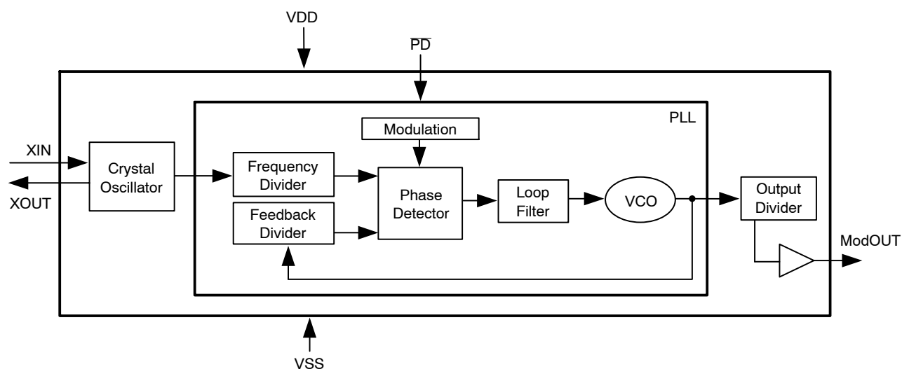
Figure 1. Block Diagram
