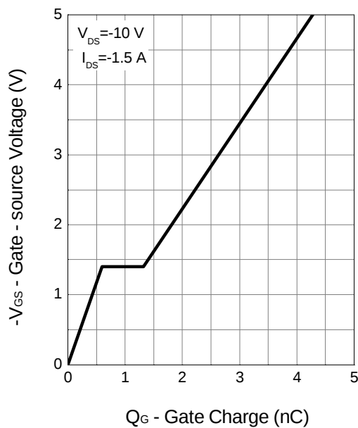
Gate Charge
