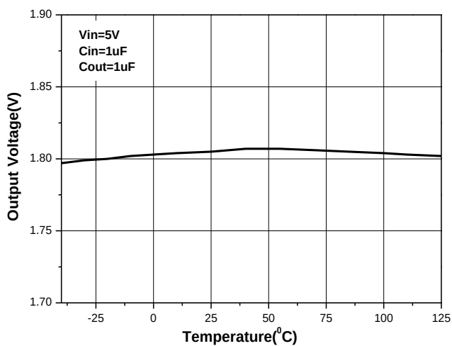
Figure 12. Temperature Stability
