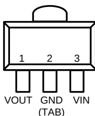
Figure 1. Pin Assignment of FP6131
