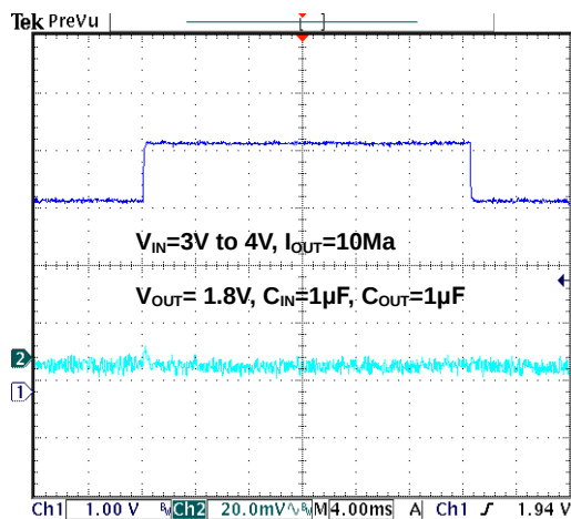
Figure 17. Line Transition Response
