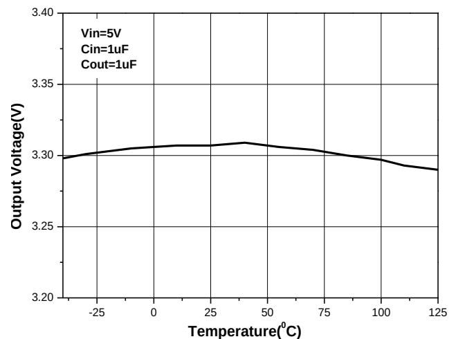
Figure 13. Temperature Stability
