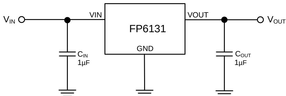
Figure 2. Typical Application Circuit of FP6131
