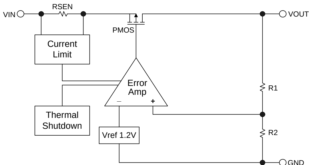
Figure 3. Block Diagram of FP6131
