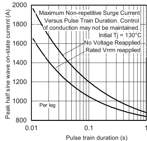
Fig. 6 - Maximum Non-Replicative Surge Current
