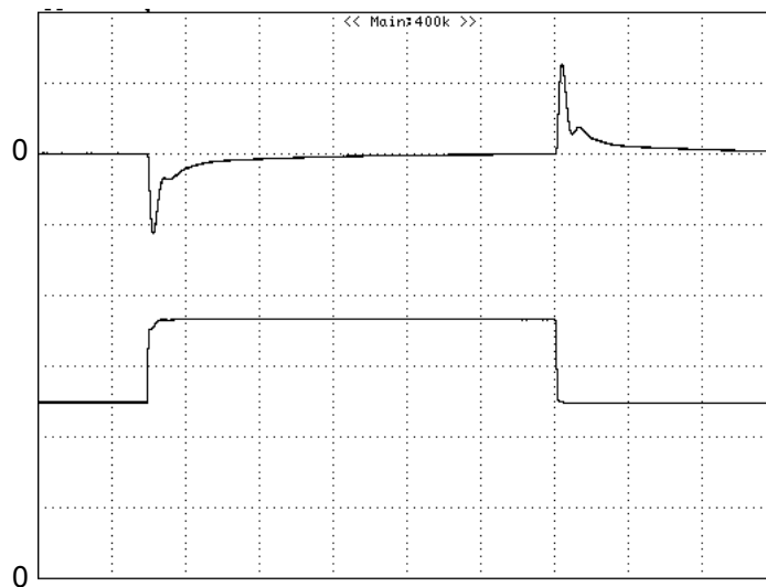
Figure 9: Output voltage response to step-change in load current (75%-50%-75% of I_o max; di/dt = 2.5A/\mu s ). Load cap: 470\mu F , 35m\Omega ESR solid electrolytic capacitor and 1\mu F ceramic capacitor. Top Trace: V_{out} (50mV/div, 200us/div), Bottom Trace: I_{out} (5A/div). Scope measurement should be made using a BNC cable (length shorter than 20 inches). Position the load between 51 mm to 76 mm (2 inches to 3 inches) from the module
