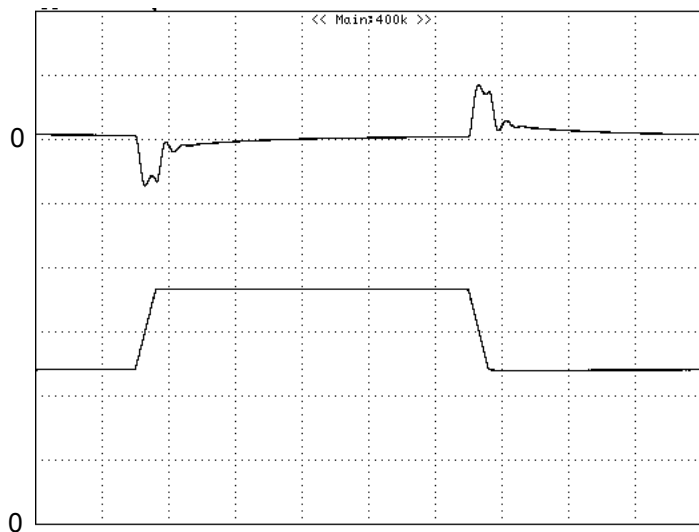
Figure 8: Output voltage response to step-change in load current (75%-50%-75% of I_o max; di/dt = 0.1A/\mu s ). Load cap: 10\mu F tantalum capacitor and 1\mu F ceramic capacitor. Top Trace: V_{out} (50mV/div, 200us/div), Bottom Trace: I_{out} (5A/div). Scope measurement should be made using a BNC cable (length shorter than 20 inches). Position the load between 51 mm to 76 mm (2 inches to 3 inches) from the module
