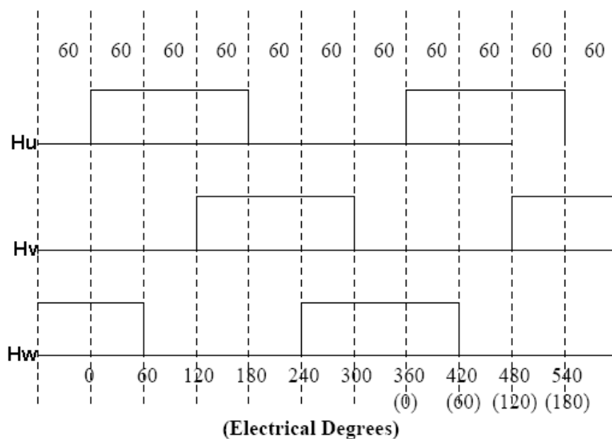
Figure 8 Hall sensor output signals
