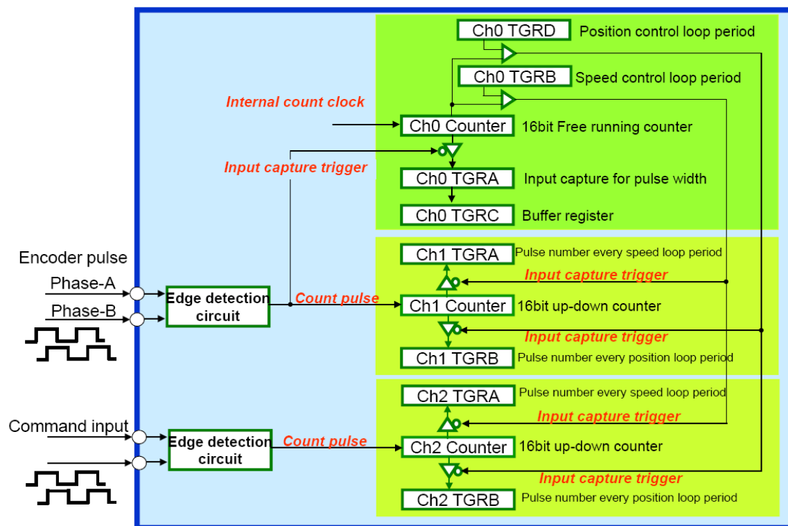
Figure 3 Encoder pulse capture in phase counting mode
