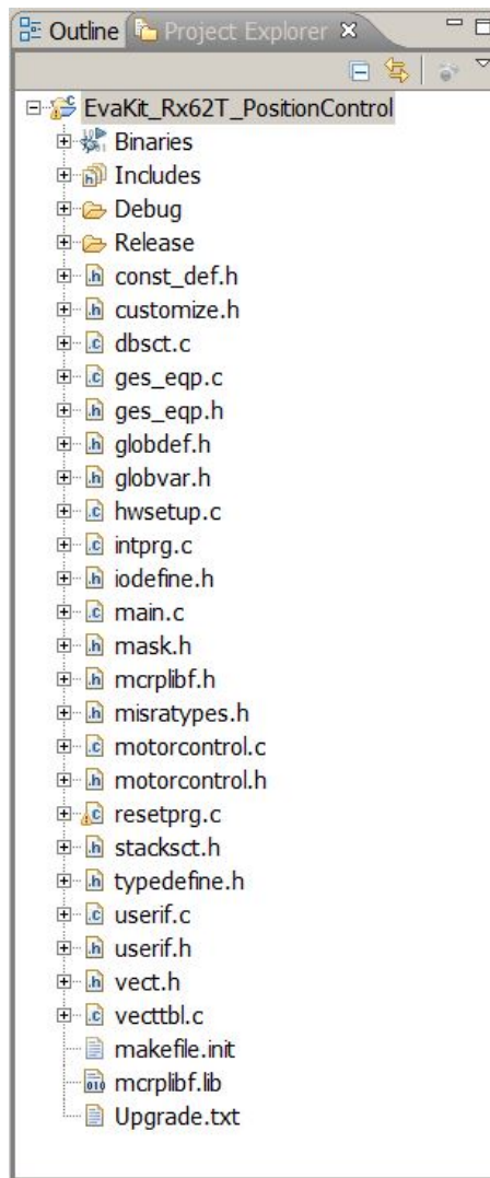
Figure 15 Encoder counting mode operation position control software workspace
