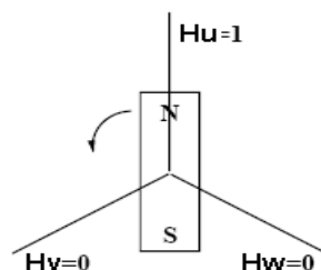
Figure 7 Hall sensors for initial rotor position
