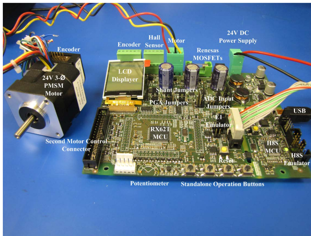
Figure 1 System hardware setup (motor and control platform)
