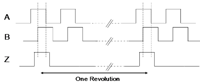
Figure 4 Relationship among the digital encoder pulses A, B and Z
