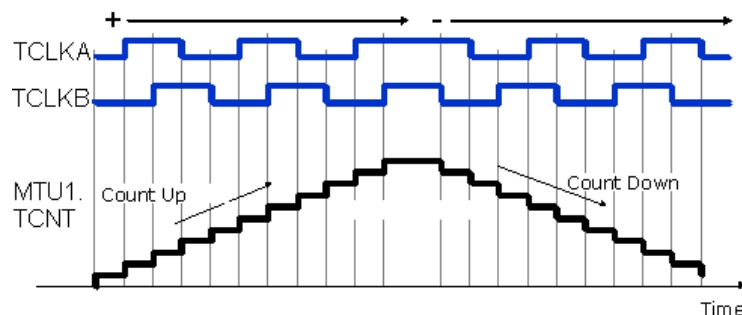
Figure 5 Encoder counting mode operation
