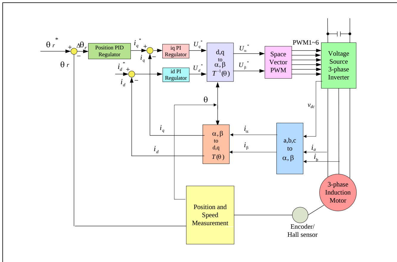
Figure 10 Position control scheme diagram
