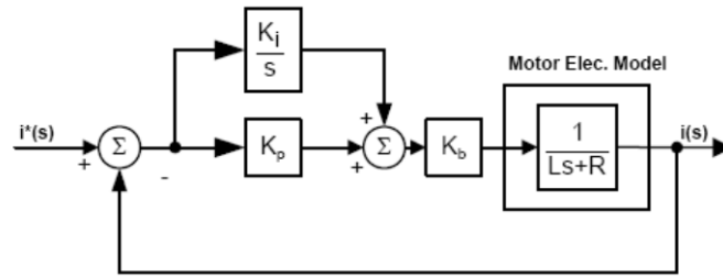
Figure 13 Current PI controller topology
