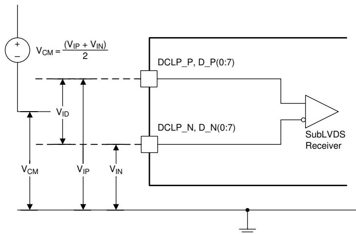
Figure 9. SubLVDS Voltage Parameters
