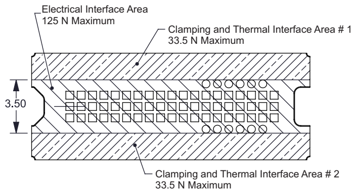
Figure 15. System Interface Loads
