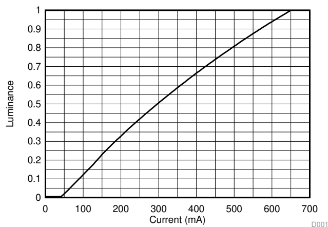
I_{LED(red)} = I_{LED(green)} = I_{LED(blue)} Figure 22. Luminance vs Current
