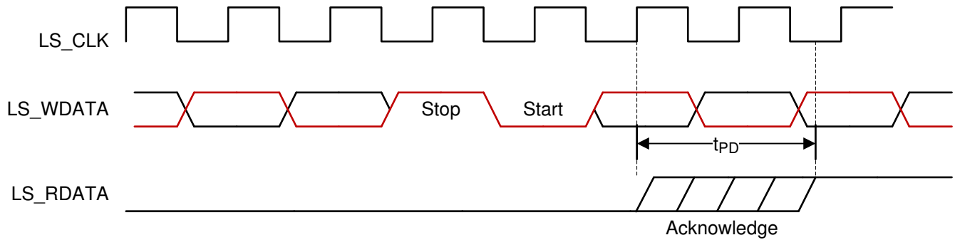
Figure 13. LPSDR Read Out
