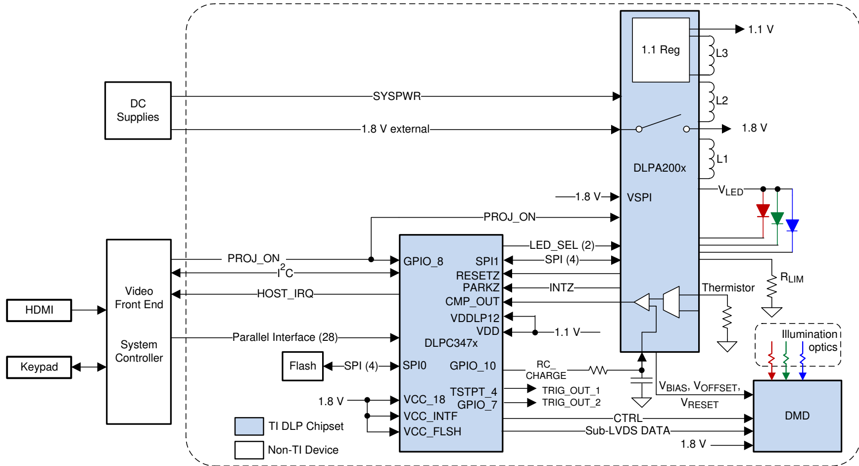
Figure 21. Typical Application
