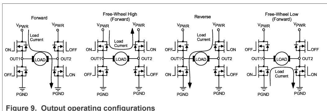
Figure 9. Output operating configurations
