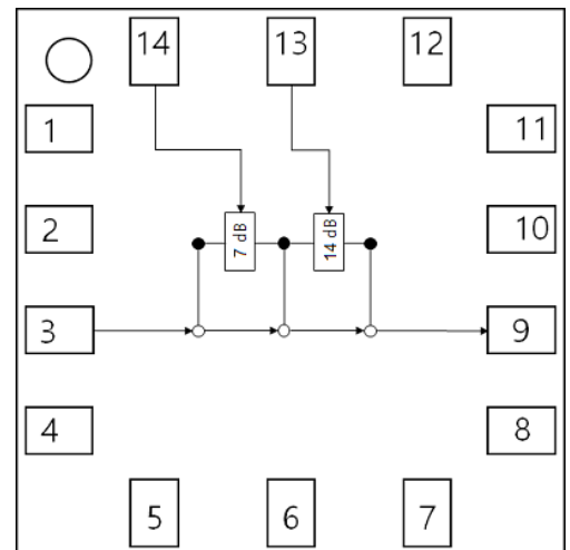
AAT2077B2 Block Diagram (X-ray view)
