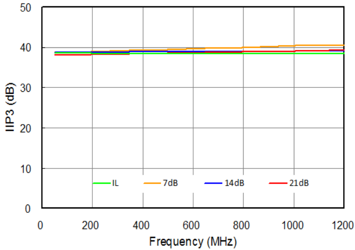
IIP3 vs. Frequency over all states
