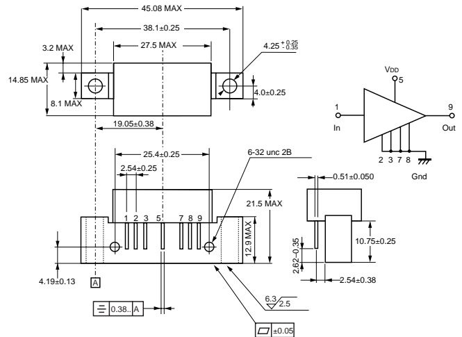
PACKAGE OUTLINE H02
