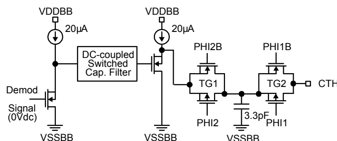
Figure 2. CTH Pin
