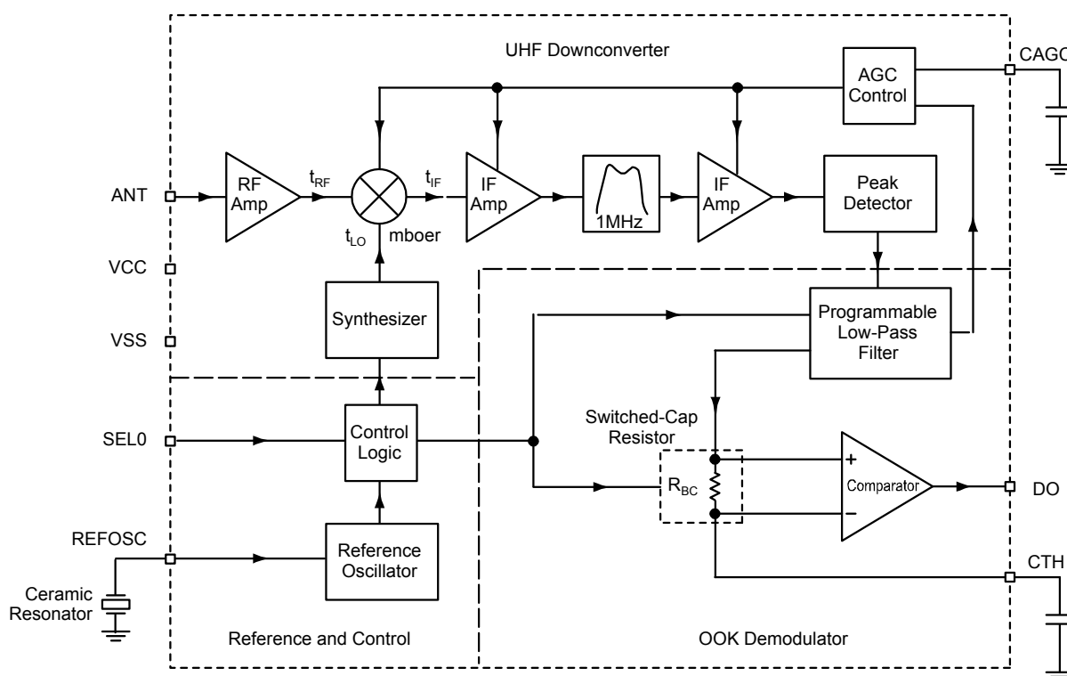
Figure 1. MICRF008 Block Diagram
