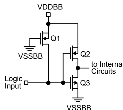
Figure 6. SEL0
