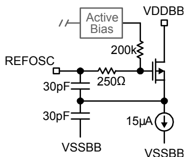
Figure 5. REFOSC Pin
