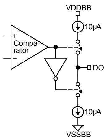
Figure 4. DO Pin
