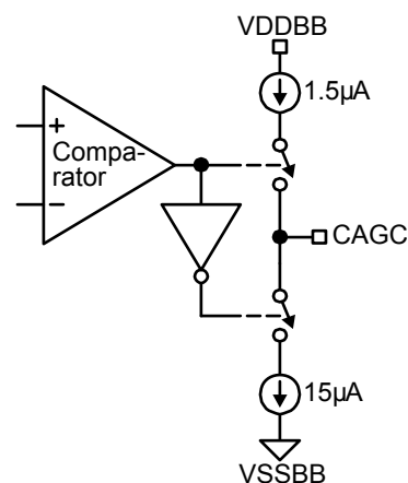
Figure 3. CAGC Pin
