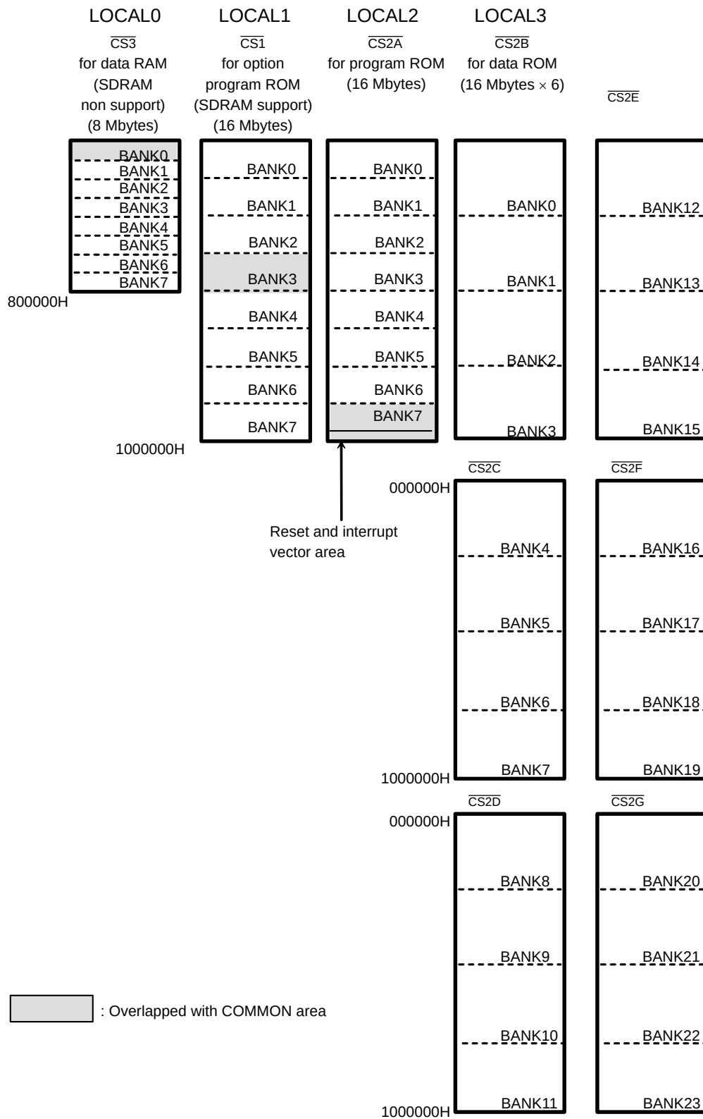
Figure 3.8.2 Physical Address Map
