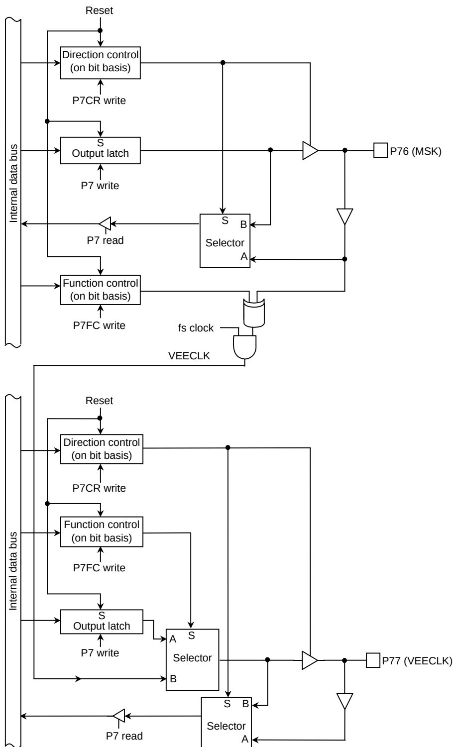
Figure 3.5.23 Port 76, 77
