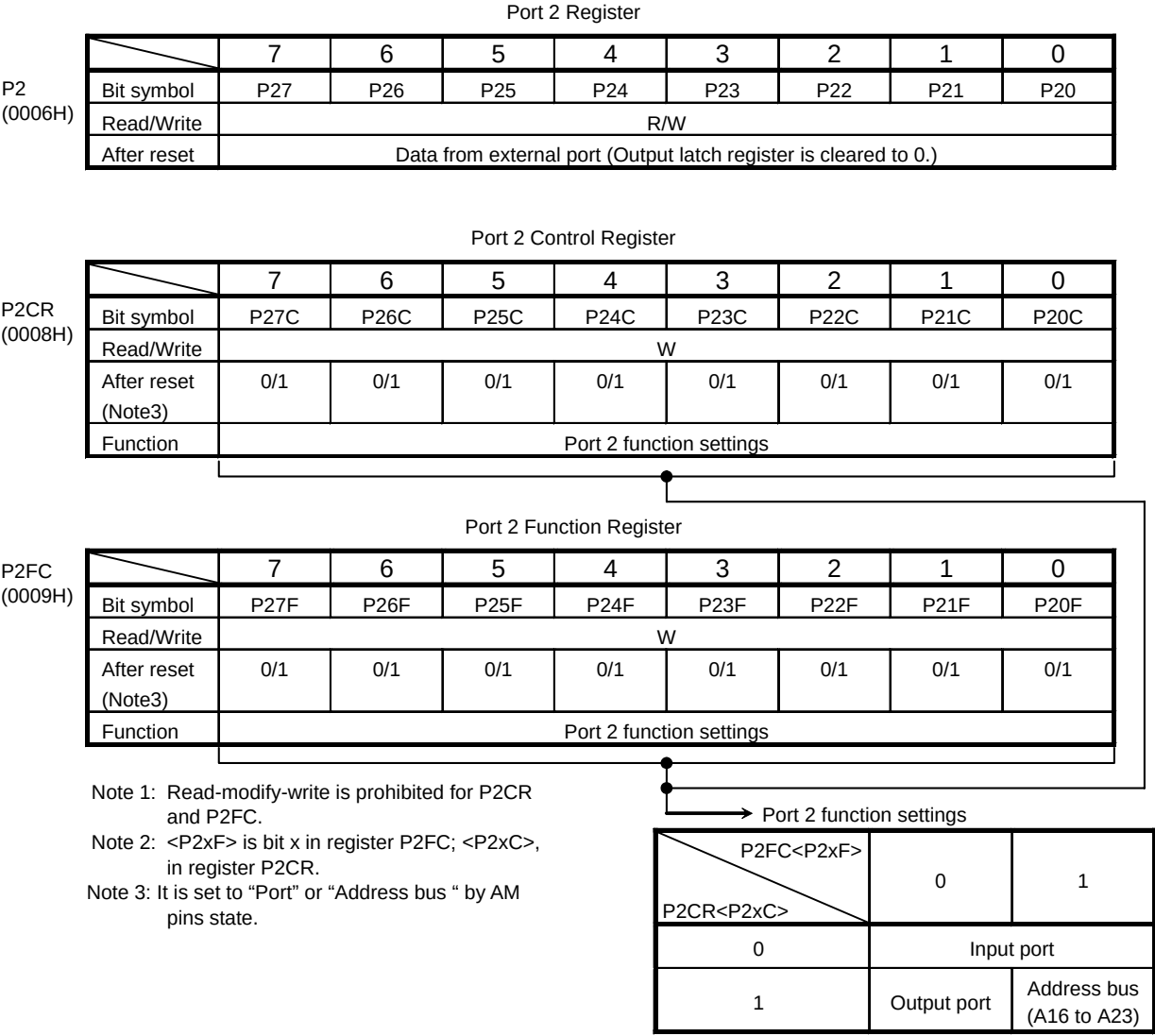
Figure 3.5.6 Register for Port 2
