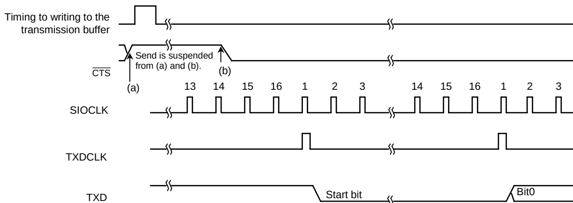
Figure 3.9.6 Handshake Function
