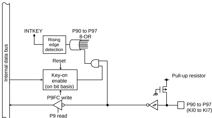
Figure 3.5.27 Port 9
