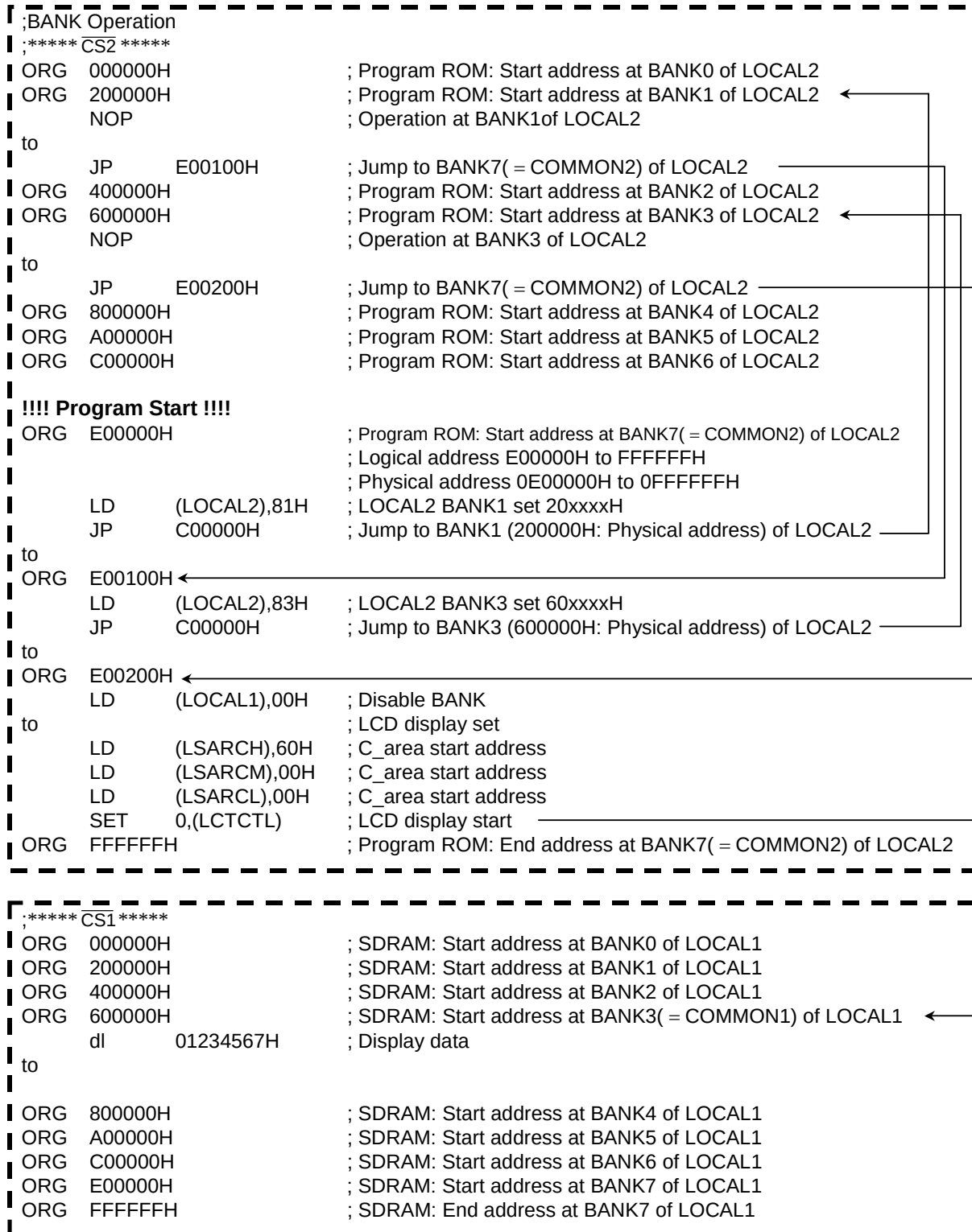
Figure 3.8.7 Bank Operation S/W Example 3
