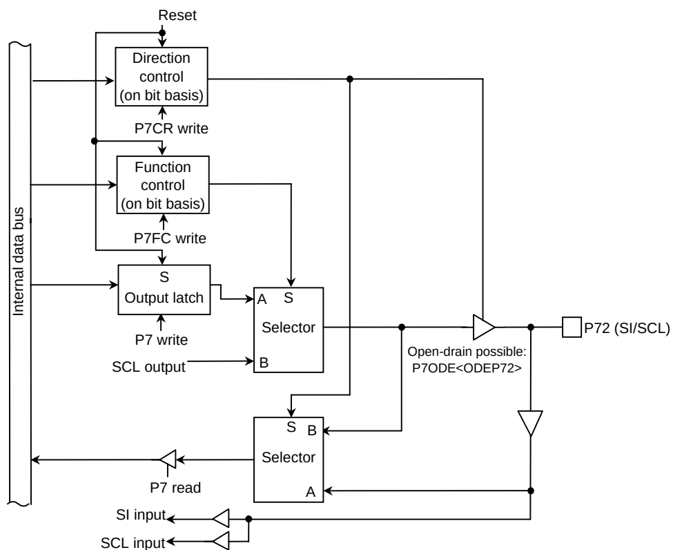
Figure 3.5.21 Port 72
