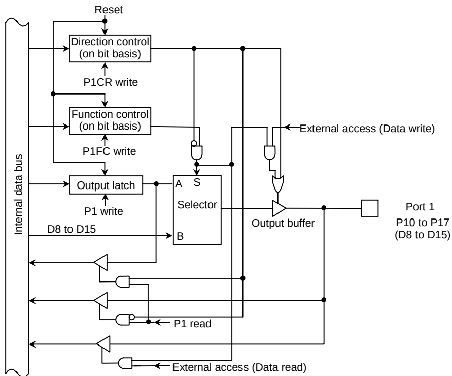
Figure 3.5.3 Port 1
