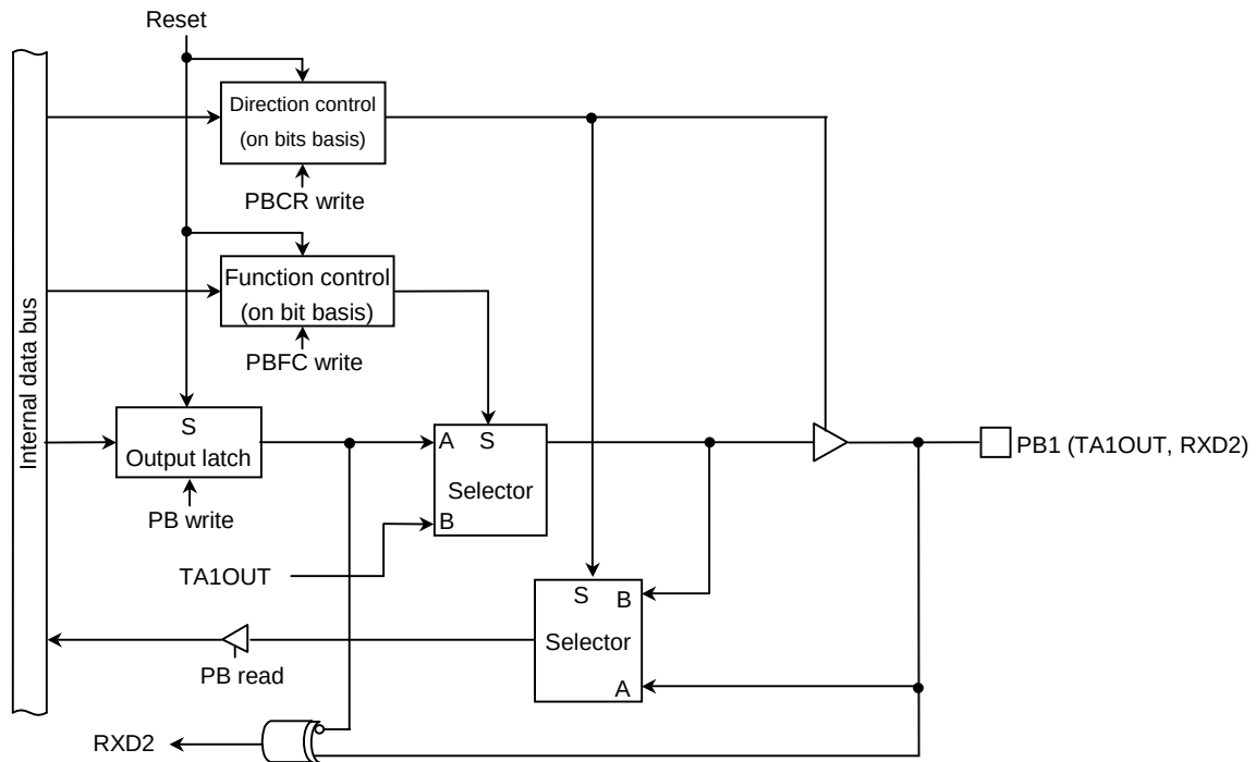
Figure 3.5.32 Port B1
