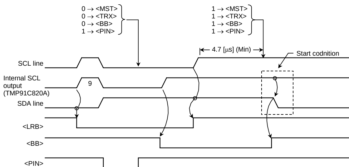
Figure 3.10.19 Timing Diagram for TMP91C820A Restart
