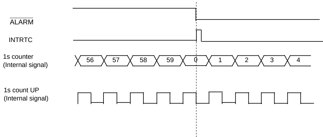
Figure 3.13.3 Timing of INTRTC and Clock data
