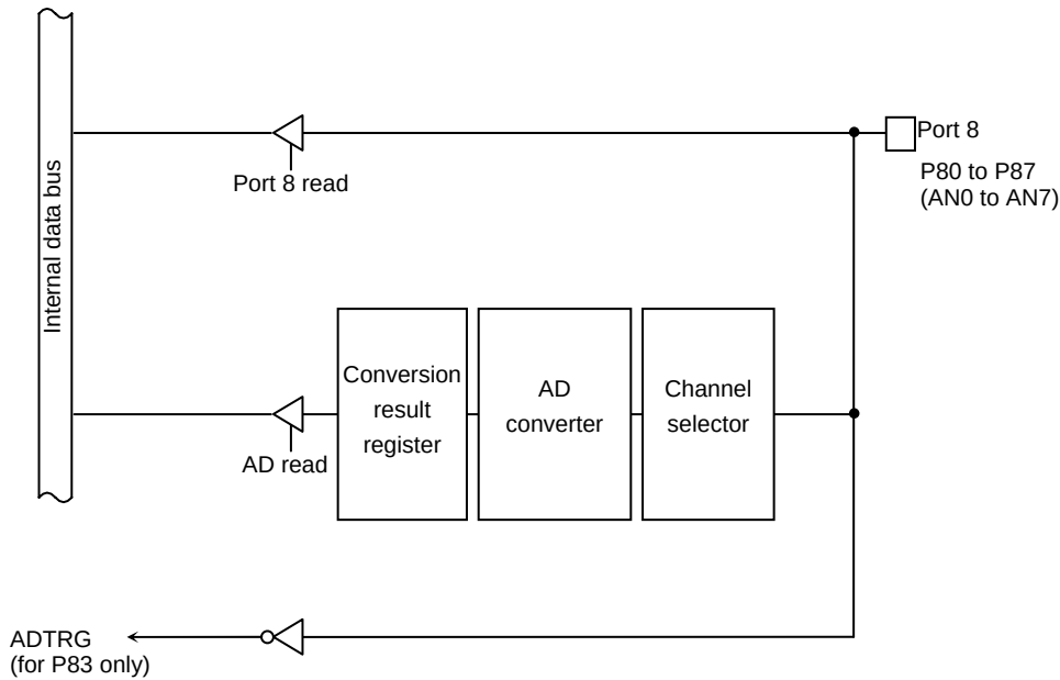
Figure 3.5.25 Port 8
