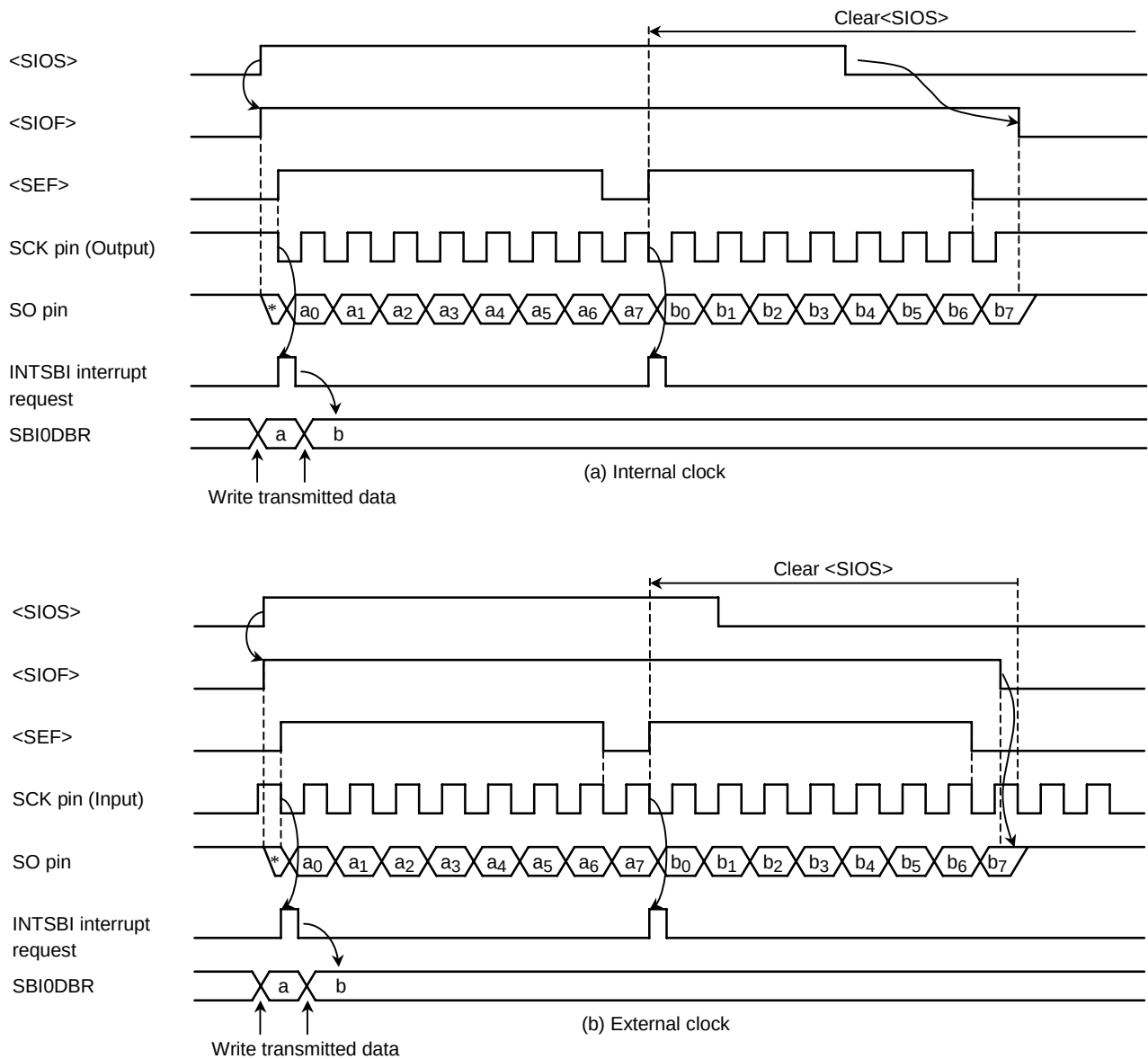
Figure 3.10.26 Transfer Mode
