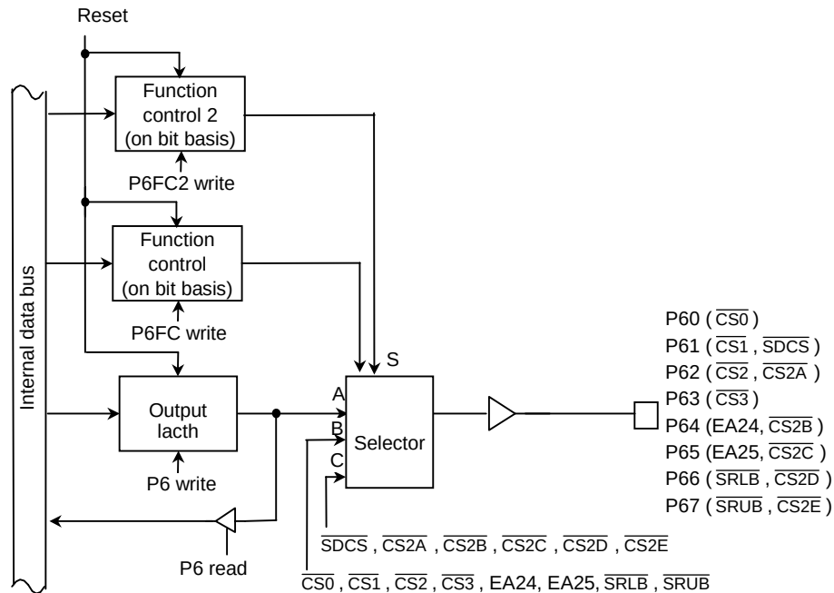
Figure 3.5.17 Port 6
