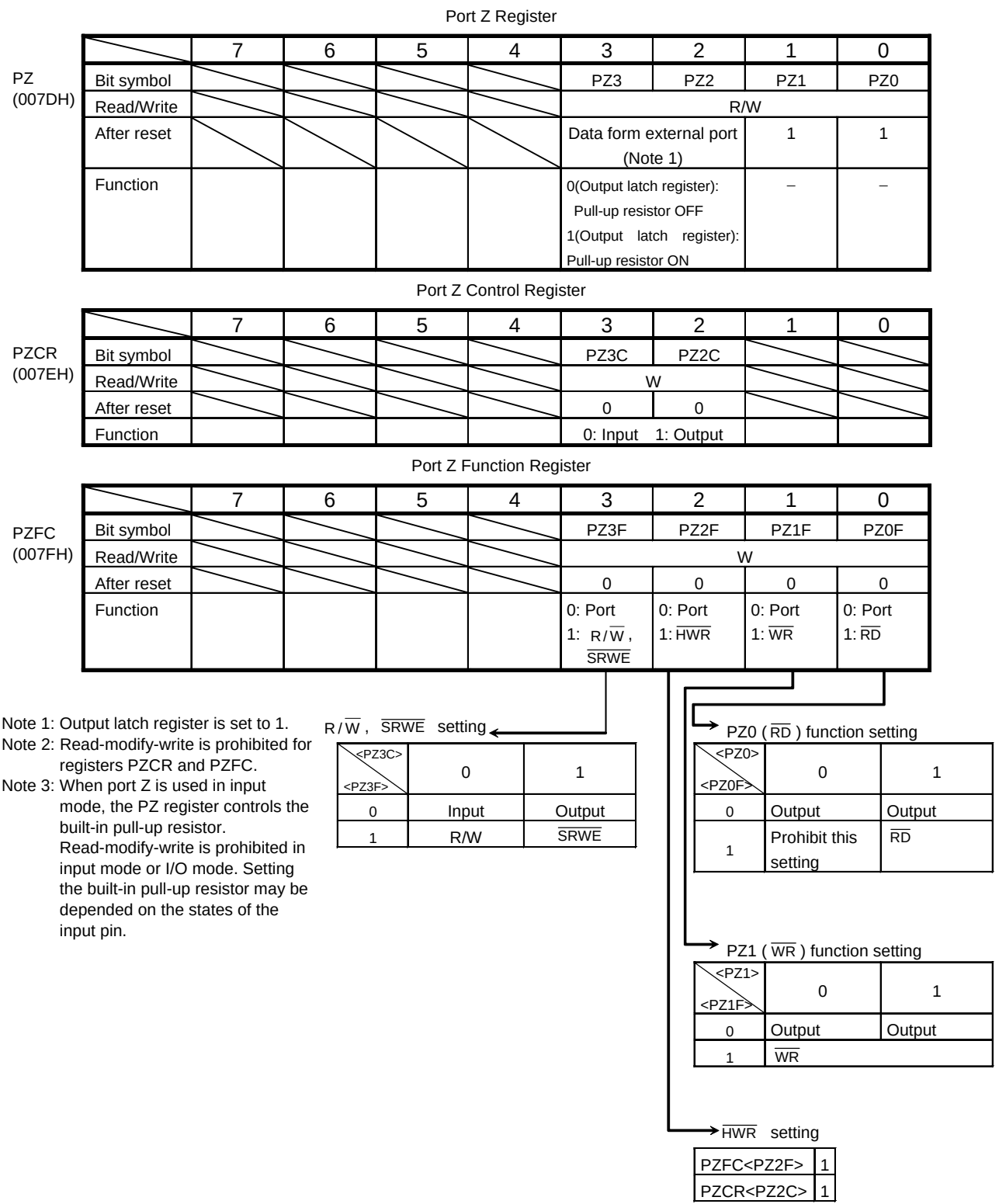
Figure 3.5.14 Register for Port Z
