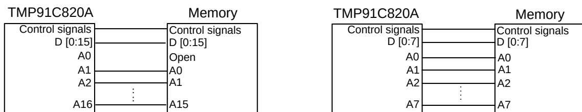
Figure 3.8.4 H/W Setting Example
