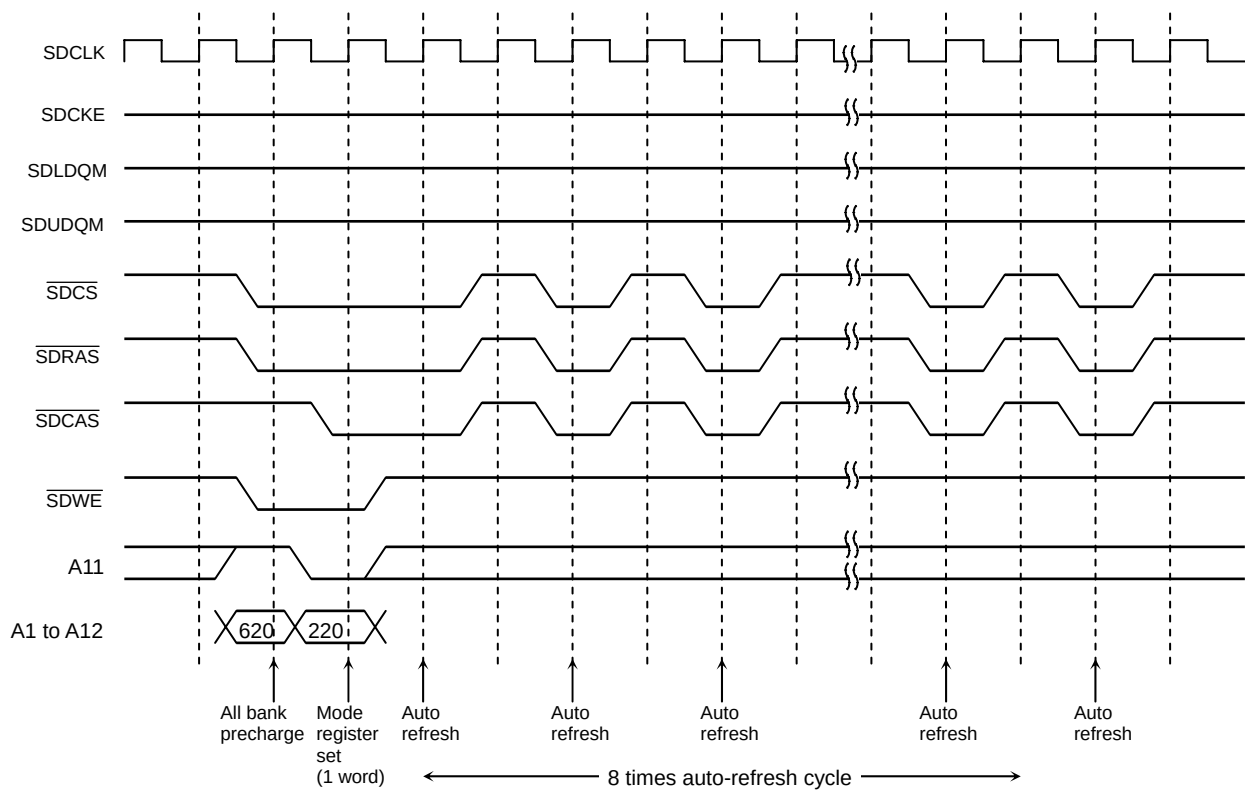
Figure 3.16.10 Initialize Cycle
