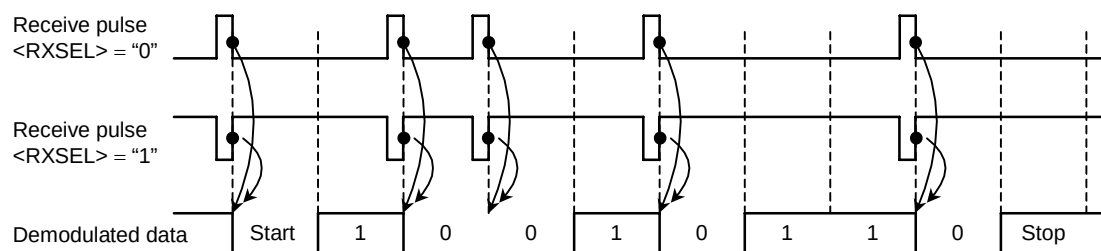
Figure 3.9.32 Receiving Example
