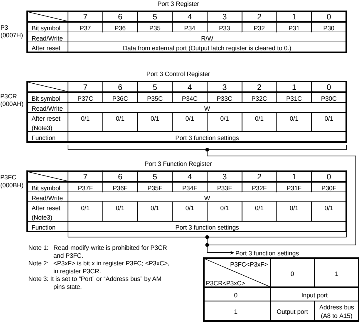
Figure 3.5.8 Register for Port 3
