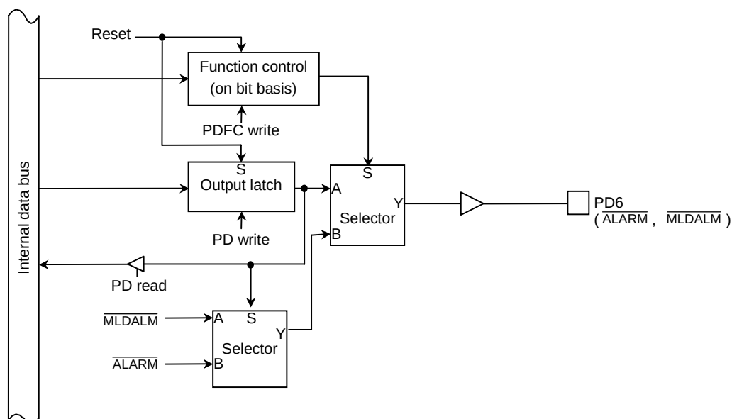
Figure 3.5.41 Port D6
