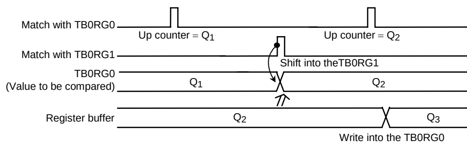
Figure 3.17.7 Operation of Register Buffer
