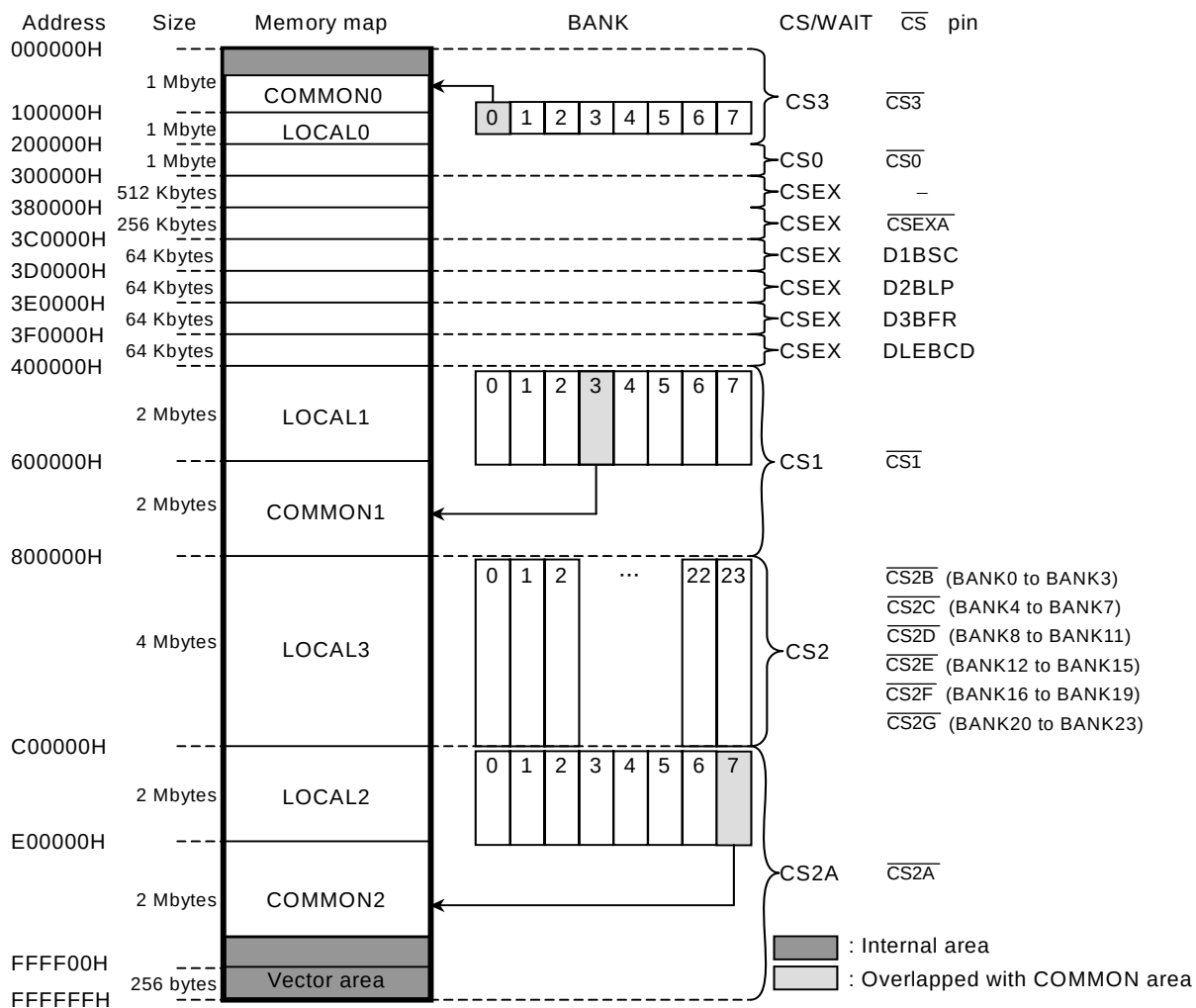
Figure 3.8.1 Recommendation Address Map (Physical address)
