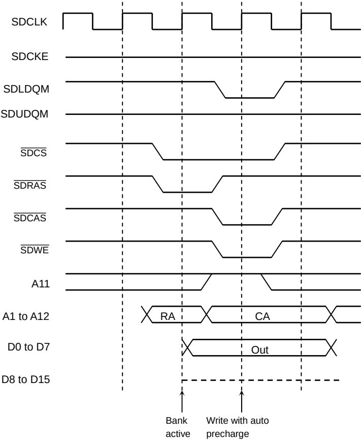
Figure 3.16.5 SDRAM Access Timing (CPU lower byte write)
