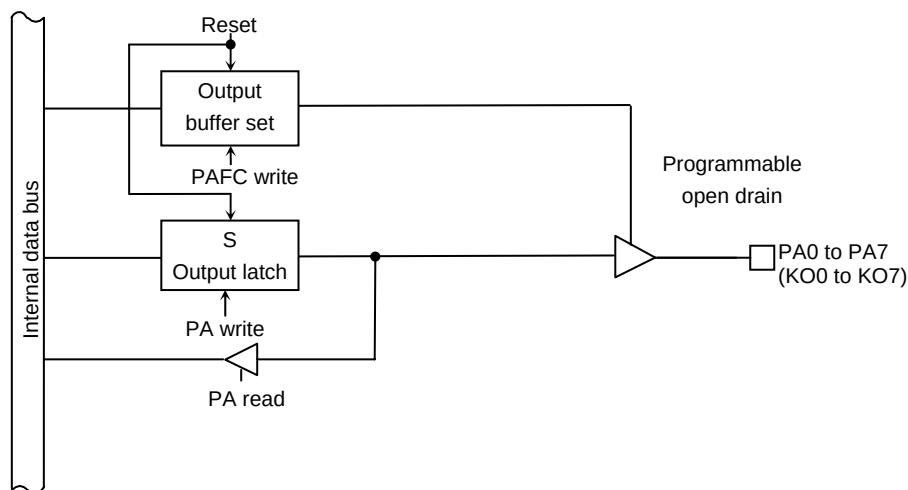
Figure 3.5.29 Port A
