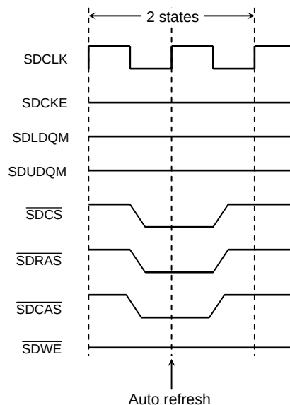
Figure 3.16.8 Refresh Cycle
