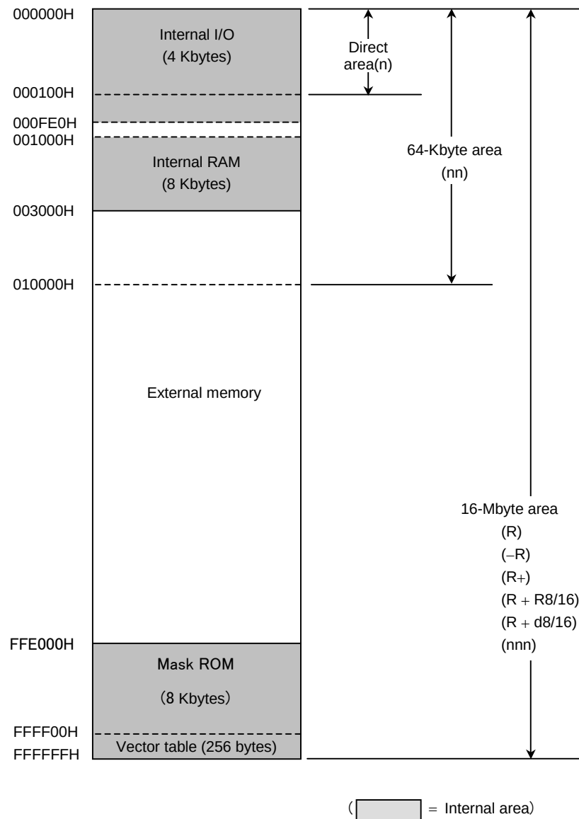
Figure 3.2.1 Memory Map
