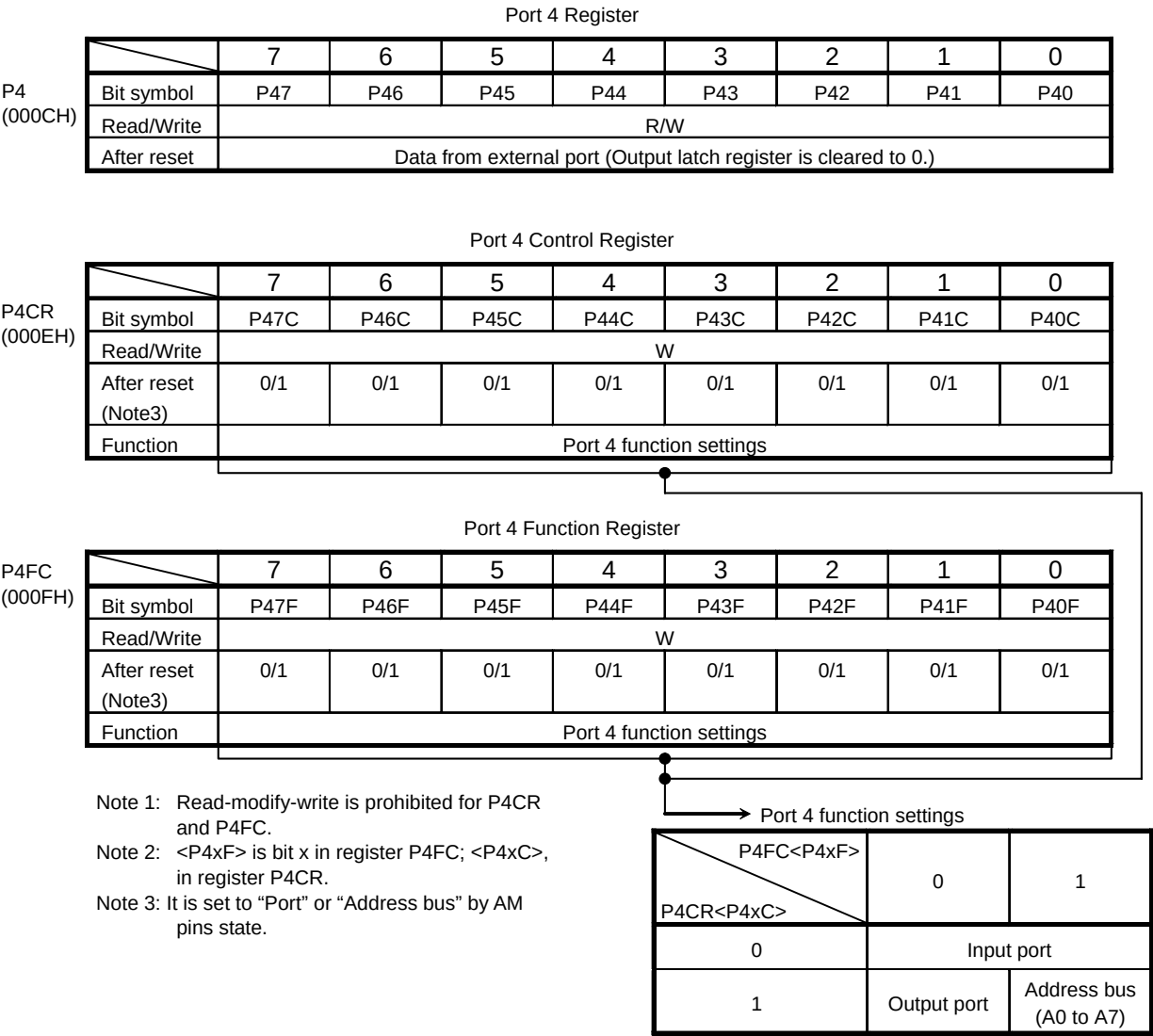
Figure 3.5.10 Register for Port 4
