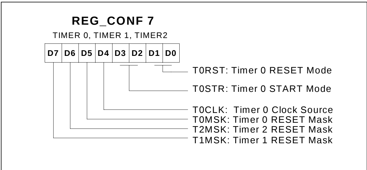
Figure 10.7 Configuration Register 7
