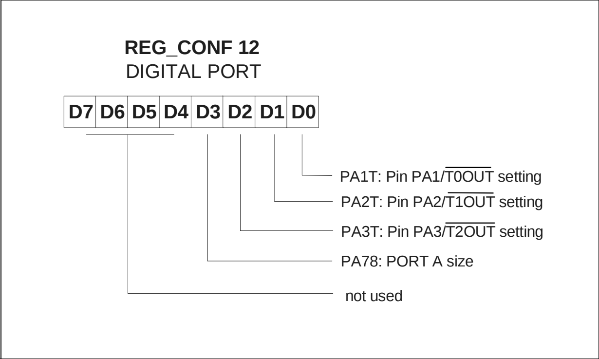
Figure 7.3 Configuration Register 12
