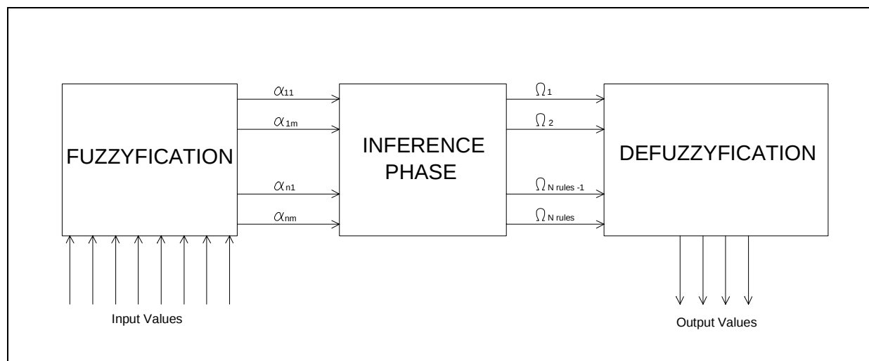
Figure 6.1 Fuzzy Inference
