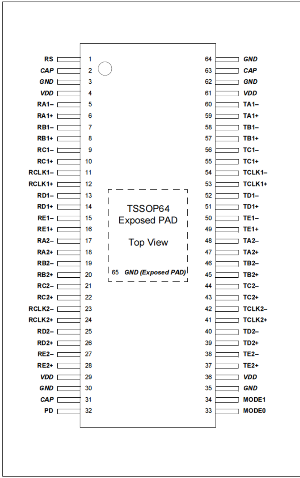
Figure 2. Pin Diagram
