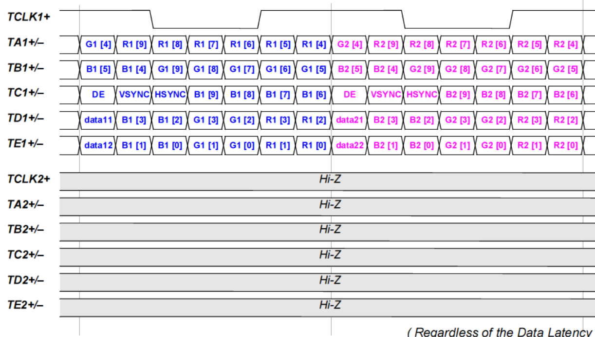
Figure 14-4. Data Mapping for Dual-In/Single-Out
