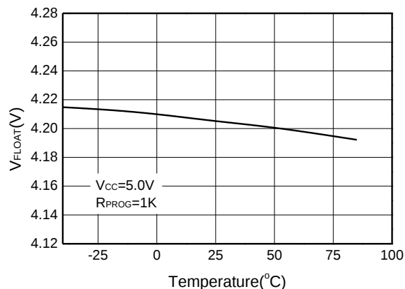
BAT Pin Output Float Voltage vs. Temperature
