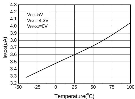
PROG Pin Pull-Up current vs. Temperature
