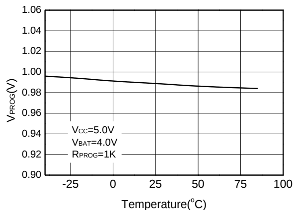
PROG Pin Voltage vs. Temperature
