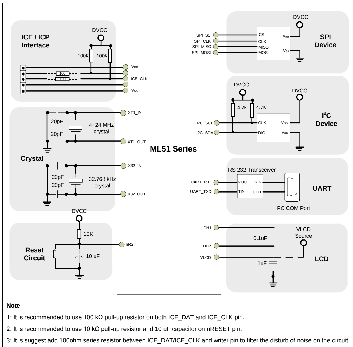
Figure 7.2-1 NuMicro® ML51/ML54/ML56 Series Peripheral interface circuit
