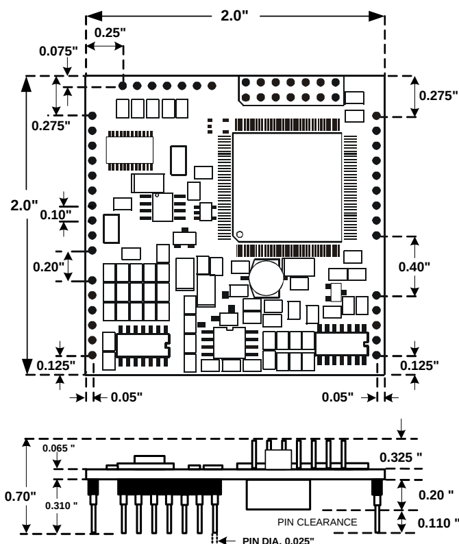
SPP-01 AND SPPDM-01 TOP VIEW AND DIMENSIONS All normal pin spacing 0.10"
