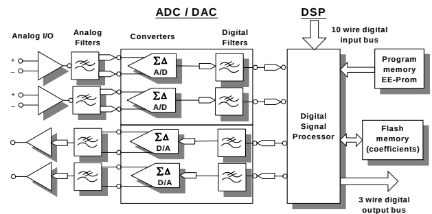
SPPDM-01 Block diagram
