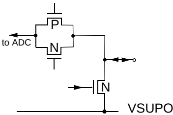
Fig. 4-9: Input/Output pin 16 (RSW1)
