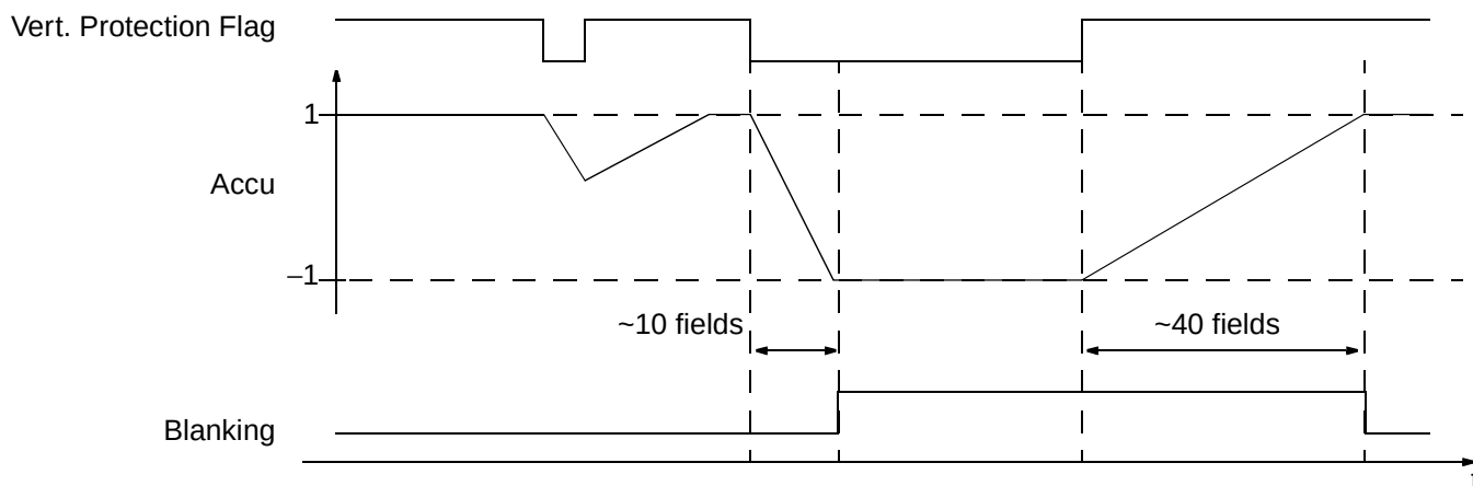
Fig. 2-17: Protection timing
