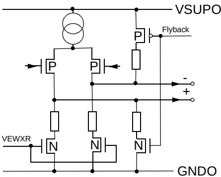
Fig. 4-11: Output pins 19 and 20 (VERT+, VERT-)
