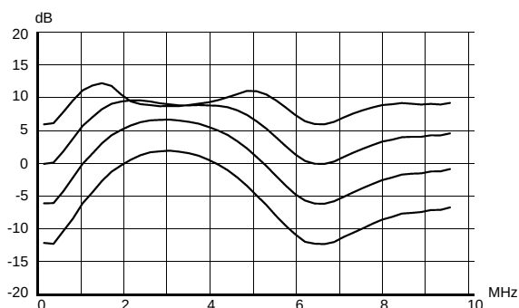
Fig. 2-1: Dynamic peaking frequency response
