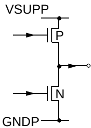
Fig. 4-4: Output pins 4 to 7 (FIFORRD, FIFORD, FIFOWR, FIFORWR)
