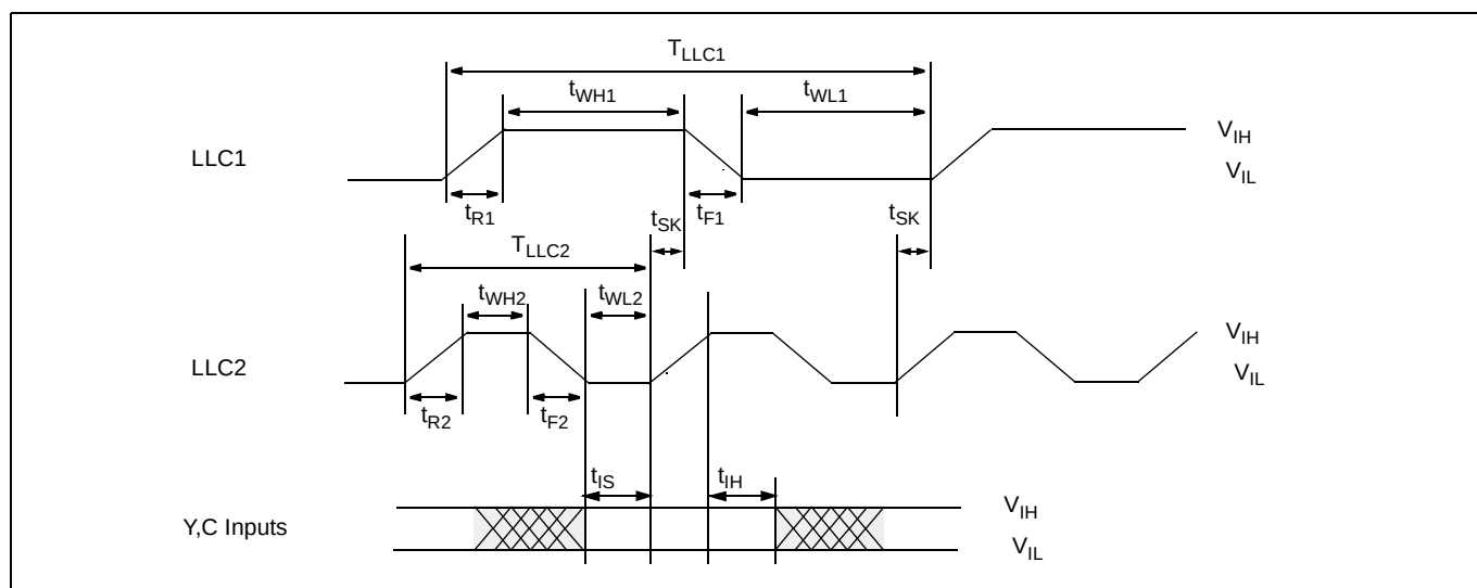
Fig. 4–21: Line-locked clock input pins and luma/chroma bus input timing
