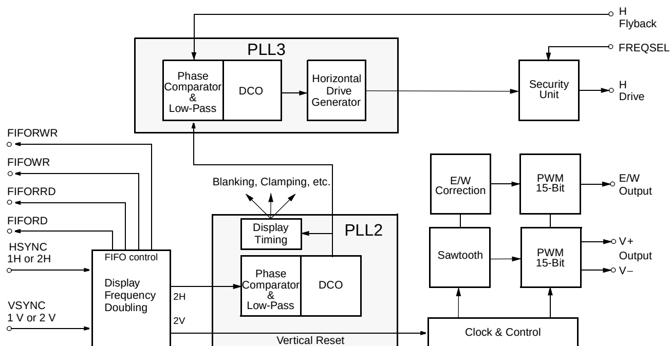
Fig. 2–13: Deflection processing block diagram
