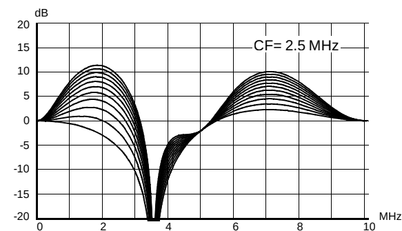
Fig. 2-2: Total frequency response for peaking filter and S-VHS, PAL, NTSC
