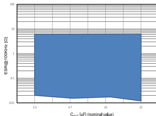
Figure 21: Stability plan (VOUT = 1.2 V)
