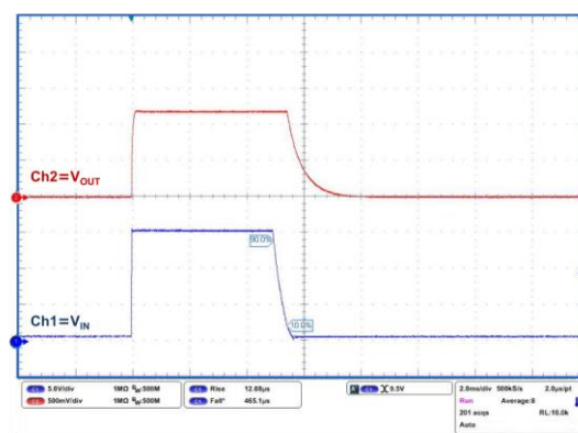
Figure 23: Turn-on time (VOUT = 1.2 V)
