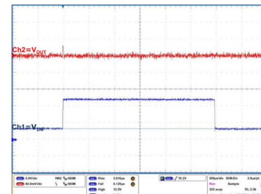
Figure 25: Line transient (VOUT = 1.2 V)
