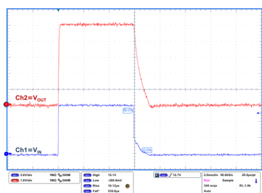
Figure 22: Turn-on time (VOUT = 5 V)
