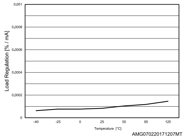
Figure 11: Load regulation vs temperature (VIN = 2.6 V, VOUT = 1.2 V, IOUT = 10 to 1200 mA)
