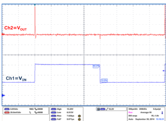
Figure 24: Line transient (VOUT = 5 V)
